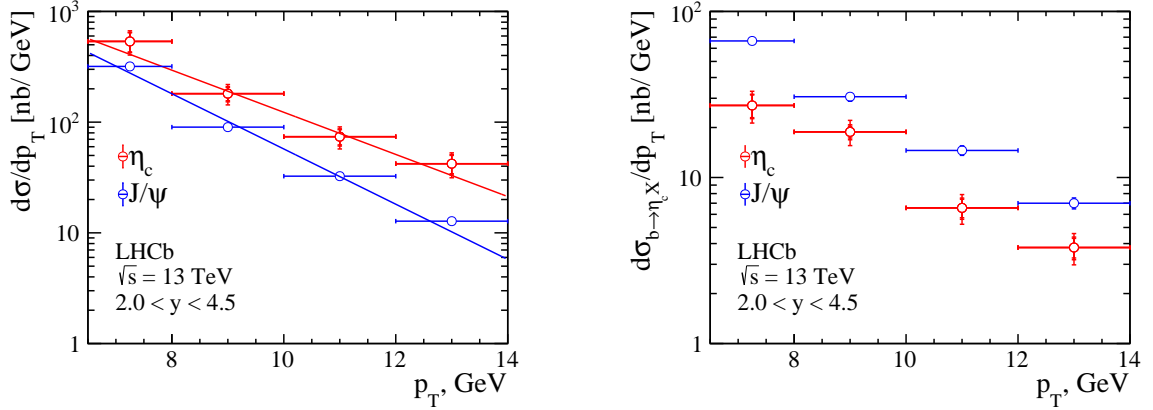
(a) Prompt-production cross section from t_z -fit technique. The results of the fits by exponential functions are overlaid. (b) Production in inclusive b -decays from separation technique .
