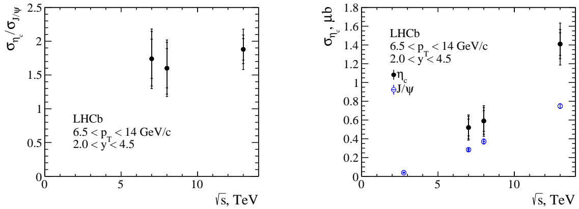
(a) Relative \eta_c prompt production cross section.
