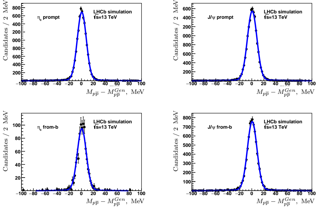
Figure 5.2: Distribution of the M_{p\bar{p}} - M_{p\bar{p}}^{Gen} value in the MC samples: prompt \eta_c (top left), prompt J/\psi (top right), \eta_c from b -decays (bottom left) and J/\psi from b -decays (bottom right). The solid blue lines represent a simultaneous fit by a double Gaussian function to all four MC samples.
