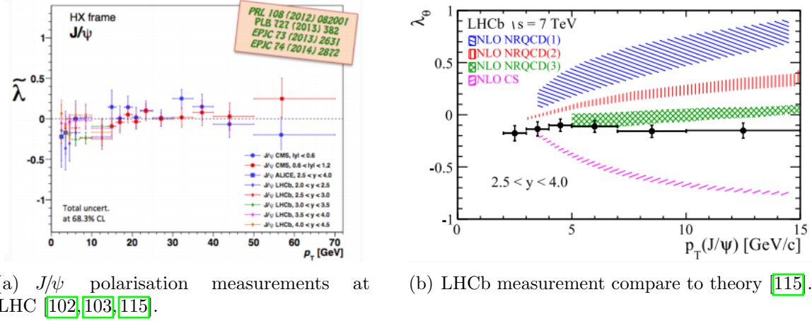
Figure 2.8: J/\psi polarisation ( \lambda_\theta ) measurements at LHC as a function of p_T .
