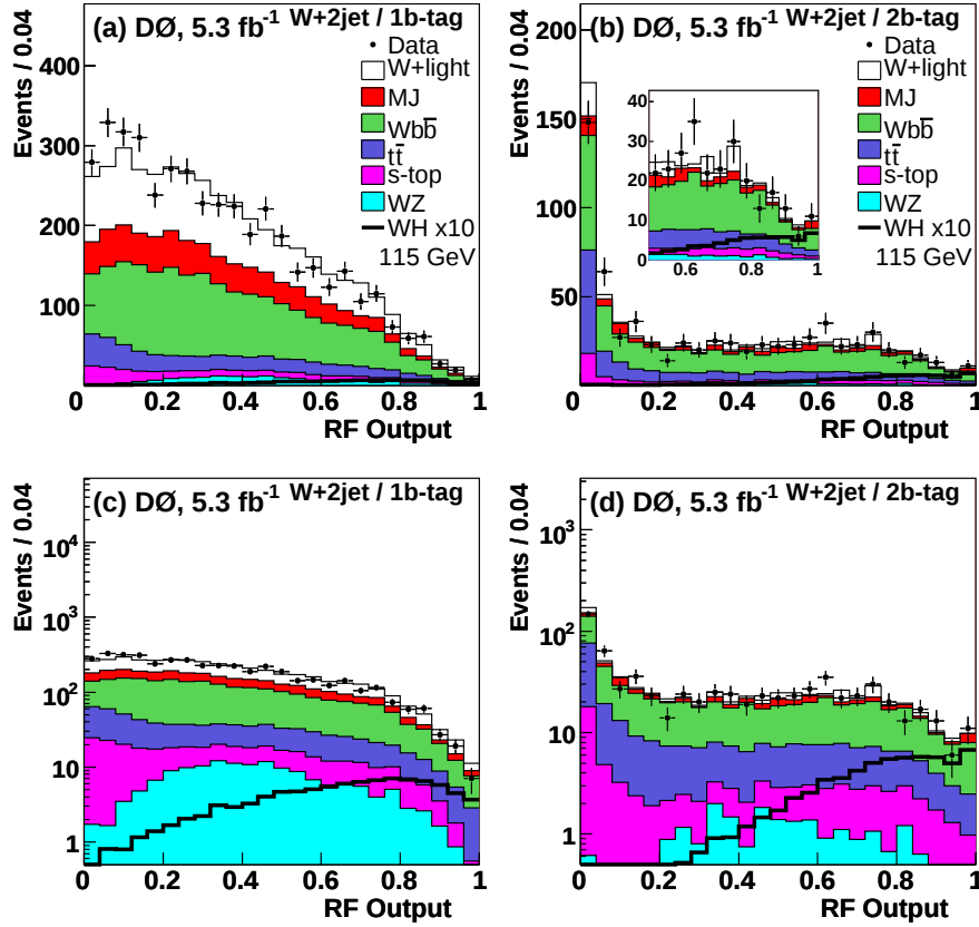
FIG. 10: [color online] Output RF distributions on linear and logarithmic scales for (a), (c) single (1b-tag) and (b), (d) two-b-tagged W+2 jet events. The expectation for signal at M_H = 115 GeV (solid black line) is scaled by a factor of ten.
