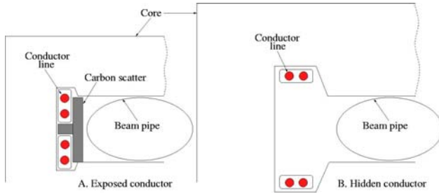
Figure 3: Options for conductor placement within a core
