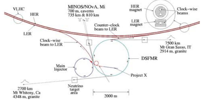
Figure 1: Outline of proposed FNAL accelerator complex
