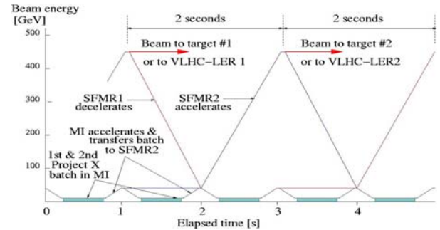
Figure 2: Time sequence for beam stacking, ramping and extraction to neutrino production targets or to LER rings.
