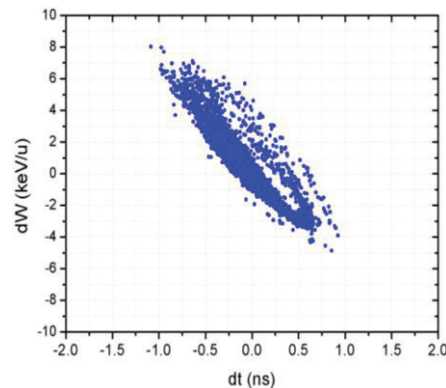
Figure 7: Simulated beam longitudinal phase space of \text{H}_2^+ beam after the RFQ.
