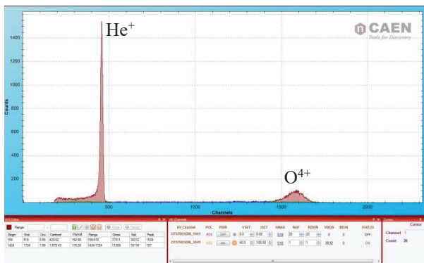
Figure 8: Measured energy spectrum for both \text{He}^+ and \text{O}^{4+} with the SiD.
