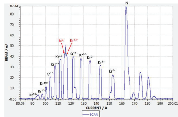
Figure 9: Measured charge state distribution after the source.
