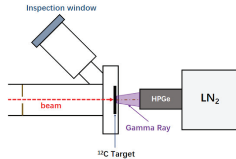
Figure 5: A sketch of experimental setup.
