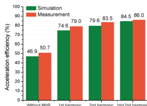
Figure 2: Measured and simulated acceleration efficiencies of the RFQ for \sim 100 \mu A N^{2+} beam under different MHB operation conditions.
