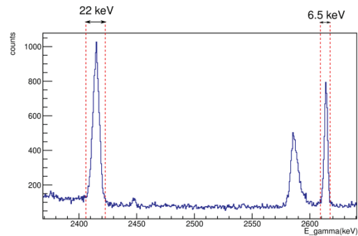
Figure 6: Measured Gamma-ray energy spectrum.
