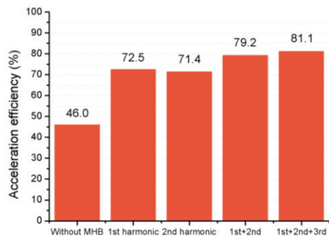
Figure 3: Measured acceleration efficiencies of the RFQ for \text{He}^{2+} beam under different MHB operation conditions.
