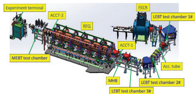
Figure 1: Layout of LEAF.
