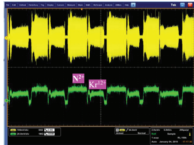
Figure 10: Measured beam currents for “ ^{86}\text{Kr}^{12+} + ^{14}\text{N}^{2+} ” “cocktail” beam after the RFQ.
