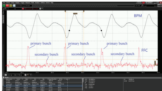
Figure 4: Measured beam longitudinal bunch shape by a Fast Faraday Cup.
