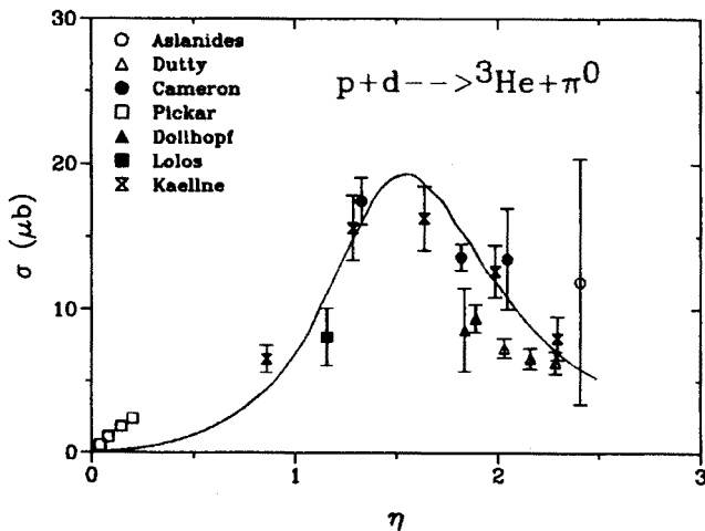
Fig. 6. Excitation function of the indicated reaction. The data are extracted total cross sections from the angular distributions given in the indicated references. The solid curve is the momentum dependence of the p + n \rightarrow d + \pi^0 reaction divided by 80 as extracted by Pickar et al.
