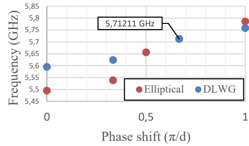
Figure 4: Dispersion diagram for both DLWG and elliptical geometries.
