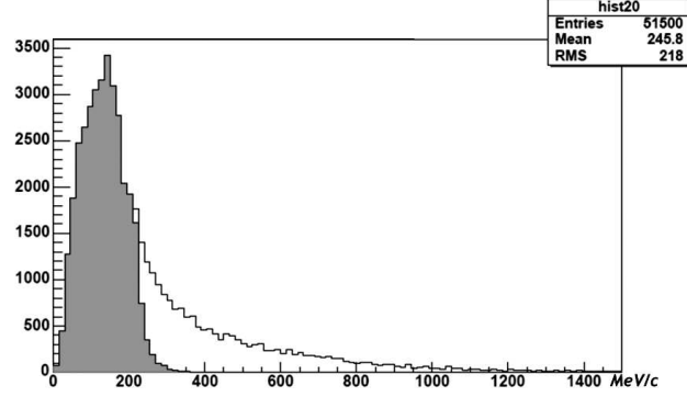
Fig. 3. Three wire criterion: visible (white) and invisible (gray) protons in the sample on the momentum histogram.
