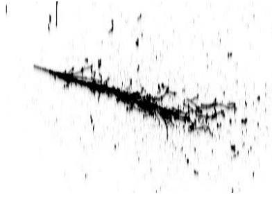
Fig. 2. An electron event with one cascade visible.
