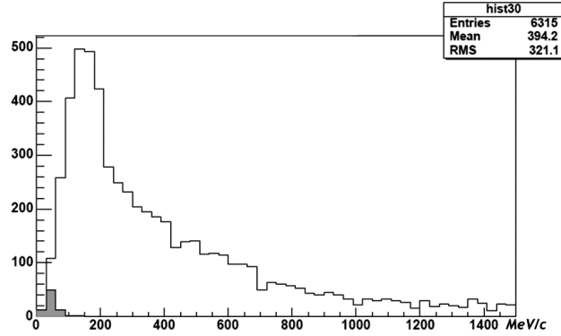
Fig. 4. Three wire criterion: visible (white) and invisible (gray) charged pions in the sample on the momentum histogram.
