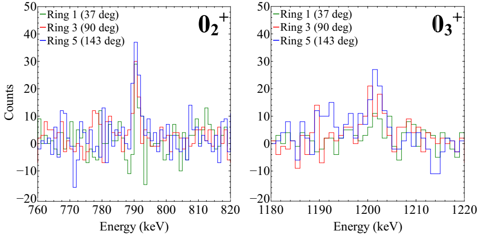
Fig. 1. Portion of the \gamma -ray energy spectra of ^{84}\text{Se} , as measured by ring 1, 3, and 5 of ROSPHERE, showing the 0_{2,3}^+ \rightarrow 2_1^+ transitions of energy 790 (left) and 1200 keV (right), depopulating the 0^+ states located at 2244 and 2654 keV, respectively. The spectra are gated on the 1454 keV, 2_1^+ \rightarrow 0_1^+ transition.
