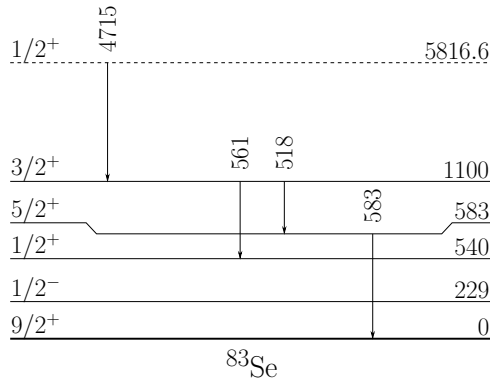
Fig. 2. Partial decay scheme of ^{83}\text{Se} . The transitions reported are those used for the angular correlation analysis.
