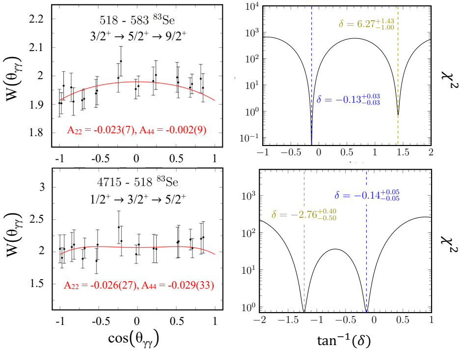
Fig. 3. Left: angular correlation for the 518–583 keV and 4715–518 keV transitions. Right: \chi^2 function for the 518 keV transition mixing ratio evaluation. The \delta values which minimize the function are reported. The picture is adapted from Ref. [11].
