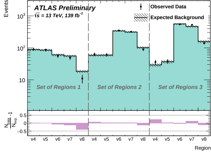
Figure 3: Expected and observed number of events in the validation regions v4-v8 for each set of regions are shown. The ratio panel shows the relative difference for each validation region.
