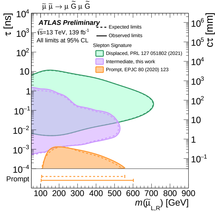
Figure 4: Expected (dashed) and observed (solid) exclusion contours for \tilde{\mu} NLSP production as a function of the left- and right-handed smuons, \tilde{\mu}_{L,R} , (top) mass and lifetime at 95% CLs, for the Displaced Slepton Signature (Phys. Rev. Lett. 127 051802 (2021) [24]), the Intermediate Slepton Signature (the result of this search in this paper) and the Prompt Slepton Signature (Eur. Phys. J. C 80 (2020) 123 [53]) reinterpretation. The lines below the graphs show the expected and observed limits from the prompt search where the smuons are assumed to be prompt.
