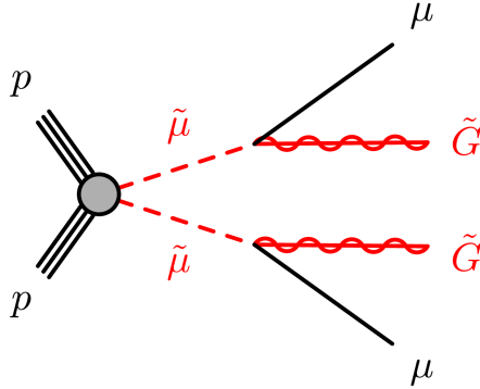
Figure 1: Decay topology of the simplified model considered where smuons ( \tilde{\mu} ) are pair produced and each smuon decays to a gravitino ( \tilde{G} ) and a muon ( \mu ).
