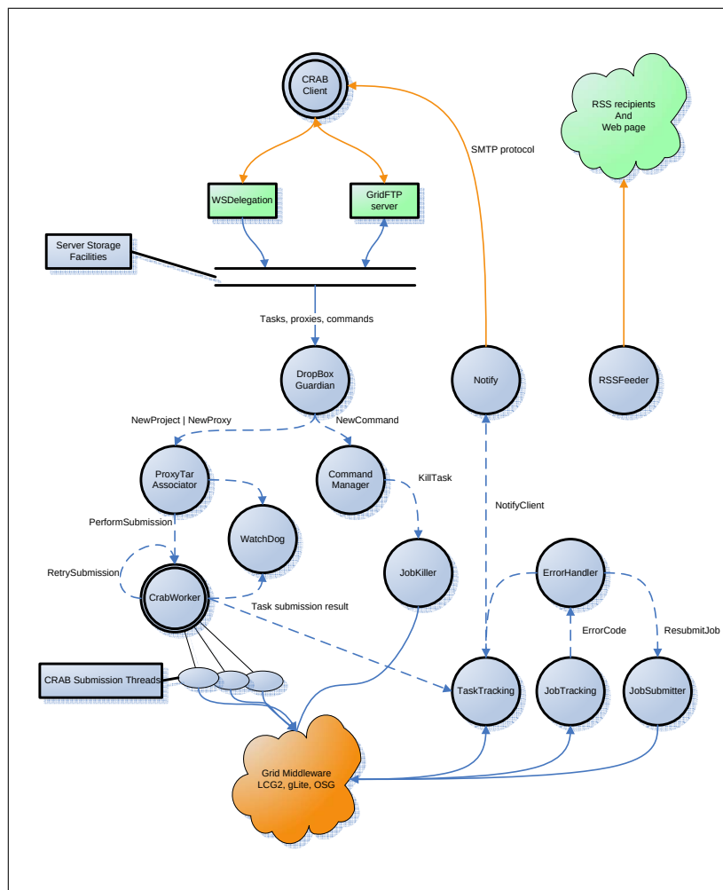
Figure 6: Dataflow diagram of the server agents
