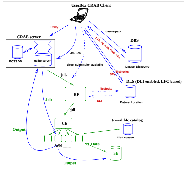
Figure 5: CRAB workflow after the adoption of the CRAB server.
