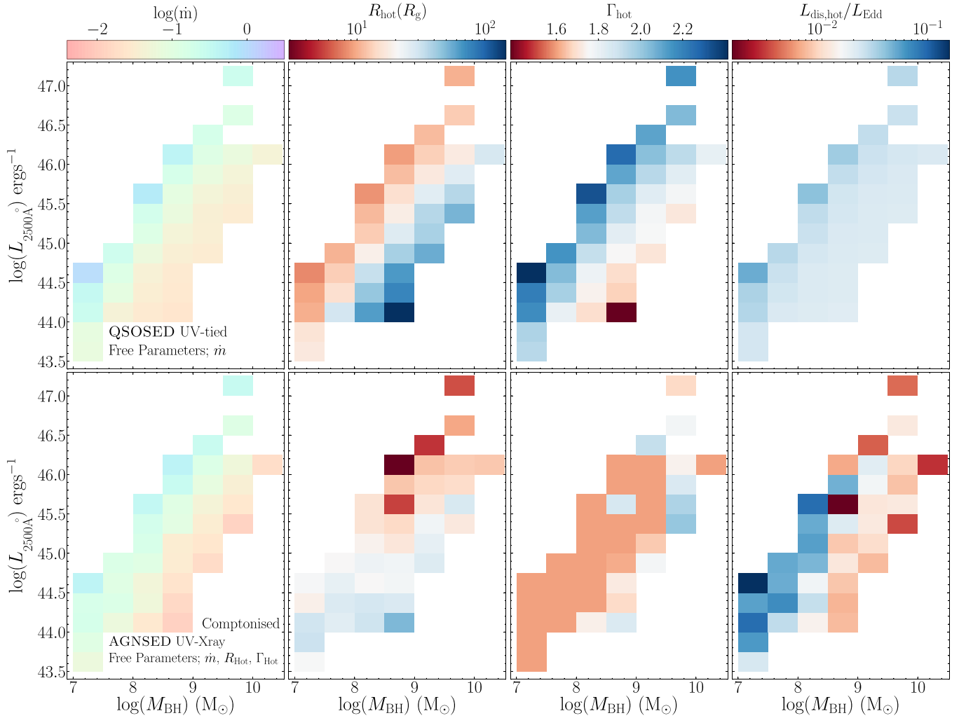
Figure 8. A comparison of the parameters of the QSOSED UV-tied fits (upper panel) and those from the AGNSEED UV-X-ray fits of Fig. 7 (lower panel). Both models have \dot{m} as a free parameter, but the AGNSEED UV-X-ray fits additionally have R_{\text{hot}} , \Gamma_{\text{hot}} , and X-ray power, L_{\text{dis, hot}}/L_{\text{Edd}} , as free parameters, whereas in QSOSED they are hardwired into the model.
