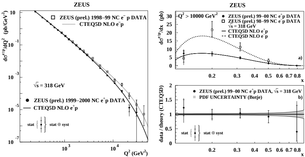
Fig. 1. The NC single differential cross sections d\sigma/dQ^2 (left) and d\sigma/dx ( Q^2 > 10000 \text{ GeV}^2 ) (top right) for e^\pm p data and SM expectation evaluated using CTEQ5D PDFs. The ratio between e^+p d\sigma/dx values and the SM prediction is also shown (bottom right), where the shaded band denotes the uncertainty of Botje's fit [3].
