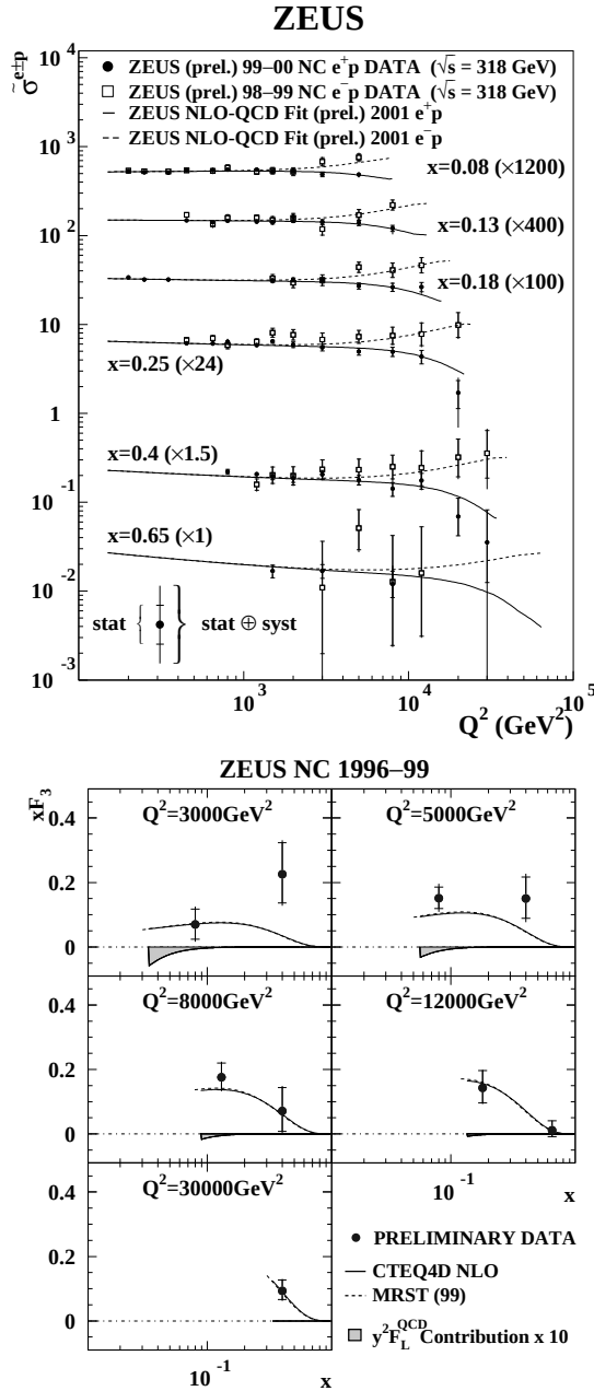
Fig. 2. The NC reduced cross section for e^\pm p data at fixed x versus Q^2 and SM expectation evaluated using the ZEUS NLO QCD fit PDFs (top). The structure function xF_3 at fixed Q^2 versus x extracted with ZEUS 1996-99 data (bottom).
