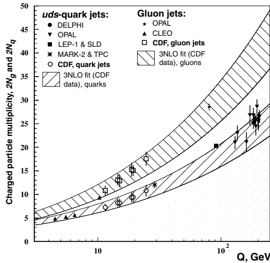
Fig. 1. Multiplicities of charged particles in gluon and quark jets vs jet hardness Q = E_{\text{jet}}\theta (see text).
