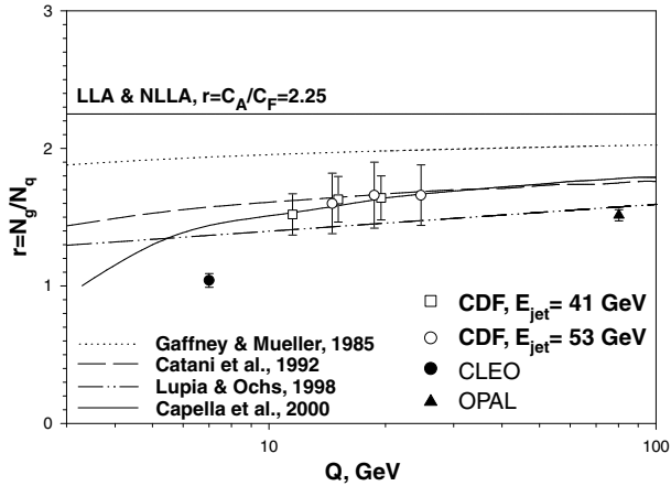
Fig. 2. Ratio of charged particles multiplicities in gluon and quark jets vs jet hardness Q = E_{\text{jet}}\theta (see text).
