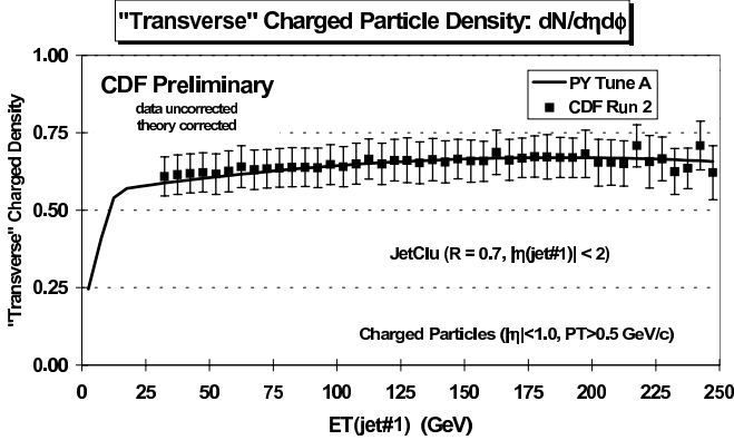
Fig. 3. Average charged particle multiplicity flow density dN/d\eta d\phi in the \phi -direction normal to the leading jet and at \eta = 0 as a function of the leading jet E_T .
