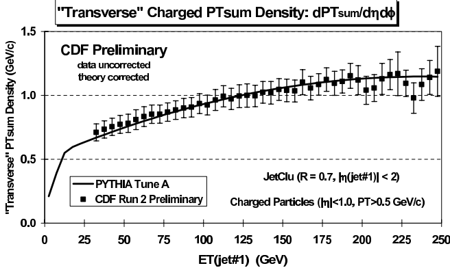
Fig. 4. Average charge particle transverse momentum flow density d(\Sigma P_T)/d\eta d\phi in the \phi -direction normal to the leading jet and at \eta = 0 as a function of the leading jet E_T .
