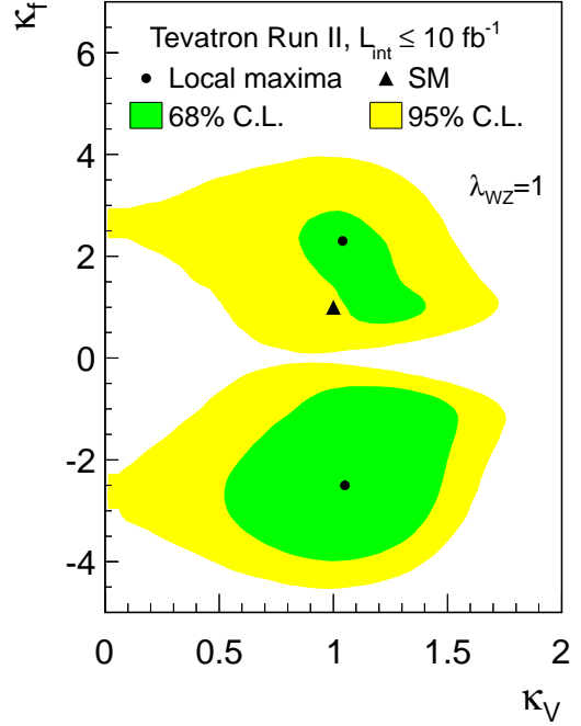
FIG. 22: (color online). Two-dimensional constraints in the (\kappa_V, \kappa_f) plane, for the combined Tevatron searches for a SM-like Higgs boson with mass 125 \text{ GeV}/c^2 assuming Custodial symmetry ( \lambda_{WZ} = 1 ). The points that maximize local posterior probability densities are marked with dots, and the 68% and 95% C.L. intervals are indicated with the dark- and light-shaded regions, respectively. The SM prediction for (\kappa_V, \kappa_f) is marked with a triangle.
