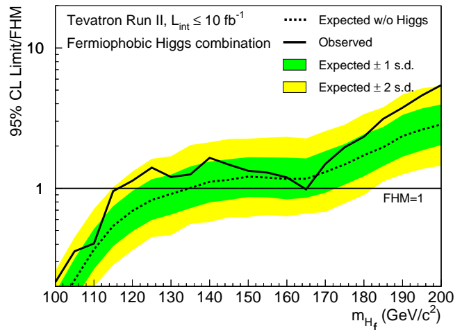
FIG. 25: (color online). Observed and median expected (for the background-only hypothesis) 95% C.L. Bayesian upper production limits expressed as multiples of the FHM cross section as a function of Higgs boson mass for the combined CDF and D0 searches. The dark and light-shaded bands indicate, respectively, the one and two s.d. probability regions in which the limits are expected to fluctuate in the absence of signal.
