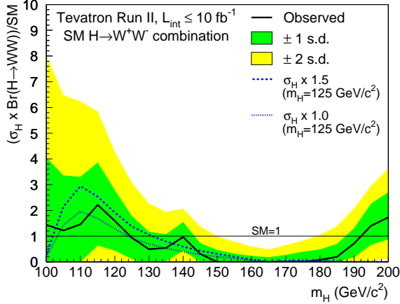
FIG. 12: (color online). The best-fit signal cross section expressed as a ratio to the SM cross section as a function of Higgs boson mass from the combination of CDF and D0's SM Higgs boson searches focusing on the H \rightarrow W^+W^- decay mode. The dark- and light-shaded bands show the one and two s.d. uncertainty ranges on the fitted signal, respectively. Also shown with blue lines are the median fitted cross sections expected for a SM Higgs boson with m_H = 125 \text{ GeV}/c^2 at signal strengths of 1.0 times (short-dashed) and 1.5 times (long-dashed) the SM prediction.
