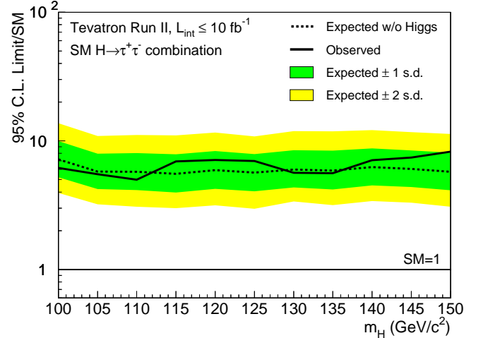
FIG. 14: (color online). Observed and median expected (for the background-only hypothesis) 95% C.L. Bayesian upper production limits expressed as multiples of the SM cross section as a function of Higgs boson mass from the combination of CDF and D0's SM Higgs boson searches focusing on the H \rightarrow \tau^+\tau^- decay mode. The dark- and light-shaded bands indicate, respectively, the one and two s.d. probability regions in which the limits are expected to fluctuate in the absence of signal.
