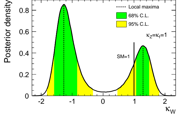
FIG. 17: (color online). Posterior probability density for \kappa_W from the combination of Tevatron searches for a SM-like Higgs boson with m_H = 125 \text{ GeV}/c^2 . The couplings of the Higgs boson to fermions and to the Z boson are assumed to be as predicted by the SM. The values that maximize local posterior probability densities are shown with dashed lines, and the 68% and 95% C.L. intervals are indicated with the dark- and light-shaded regions, respectively. The predicted SM value of \kappa_W is indicated by the solid line.
