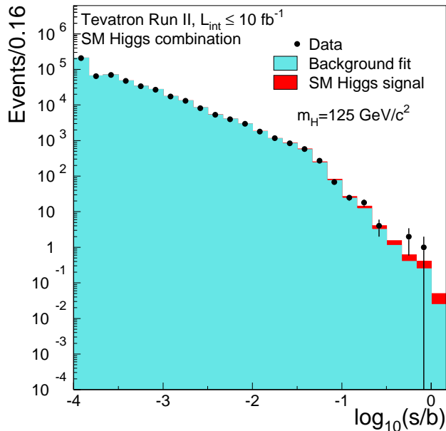
FIG. 1: (color online). Distribution of \log_{10}(s/b) , for the data from all contributing Higgs boson search channels from CDF and D0, for m_H = 125 \text{ GeV}/c^2 . The data are shown with points, and the expected signal is shown stacked on top of the backgrounds, which are fit to the data within their systematic uncertainties. The error bars shown on the data correspond in each bin to the square root of the observed data count. Underflows and overflows are collected into the leftmost and rightmost bins, respectively.
