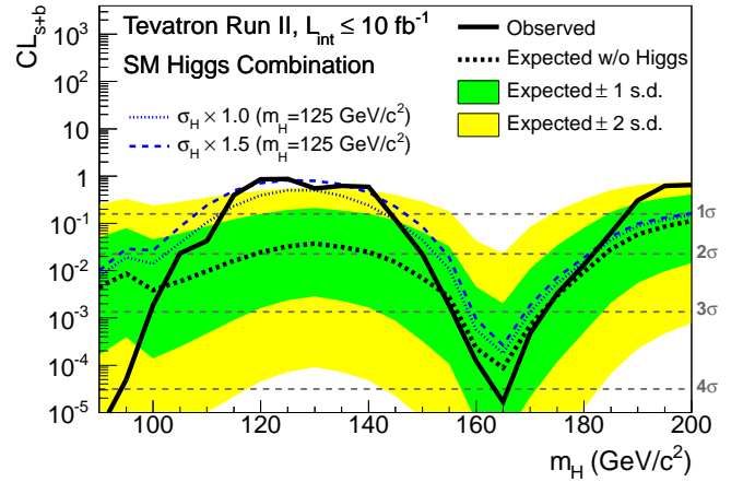
FIG. 8: (color online). The solid black line shows the signal-plus-background p -value as a function of m_H for all of CDF and D0’s SM Higgs boson searches in all decay modes combined. The dotted black line shows the median expected values assuming no SM signal is present, evaluated separately at each m_H . The associated dark and light-shaded bands indicate the one and two s.d. fluctuations of possible experimental outcomes under this scenario. The blue lines show the median expected p -values assuming the SM Higgs boson is present with m_H=125 GeV/ c^2 at signal strengths of 1.0 times (short-dashed) and 1.5 times (long-dashed) the SM prediction.
