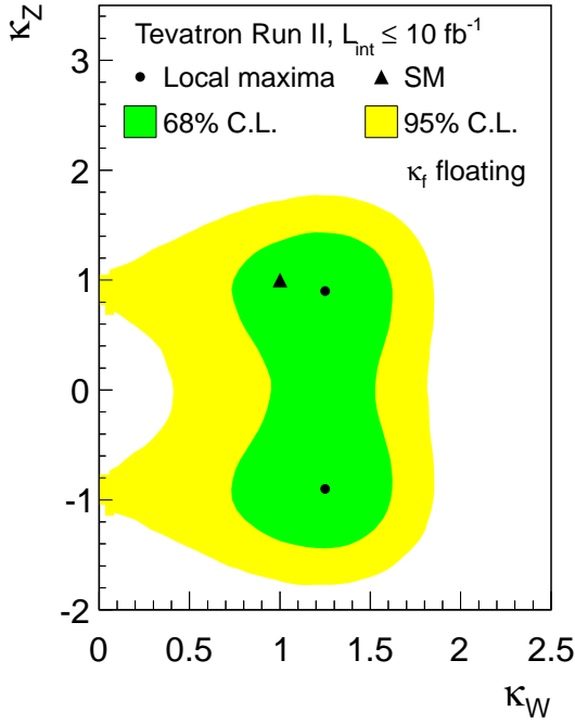
FIG. 20: (color online). Two-dimensional constraints in the (\kappa_W, \kappa_Z) plane, for the combined Tevatron searches for a SM-like Higgs boson with mass 125 \text{ GeV}/c^2 allowing \kappa_f to float. The points that maximize local posterior probability densities are marked with dots, and the 68% and 95% C.L. intervals are indicated with the dark- and light-shaded regions, respectively. The SM prediction for (\kappa_W, \kappa_Z) is marked with a triangle.
