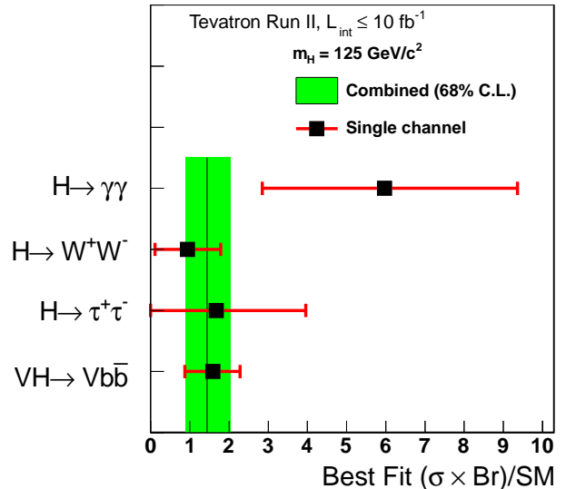
FIG. 15: (color online) Best-fit values of R = (\sigma \times \mathcal{B})/SM using the Bayesian method for the combinations of CDF and D0's Higgs boson search channels focusing on the H \rightarrow W^+W^- , H \rightarrow b\bar{b} , H \rightarrow \gamma\gamma , and H \rightarrow \tau^+\tau^- decay modes for a Higgs boson mass of 125 GeV/ c^2 . The shaded band corresponds to the one s.d. uncertainty on the best-fit value of R for all SM Higgs boson decay modes combined.
