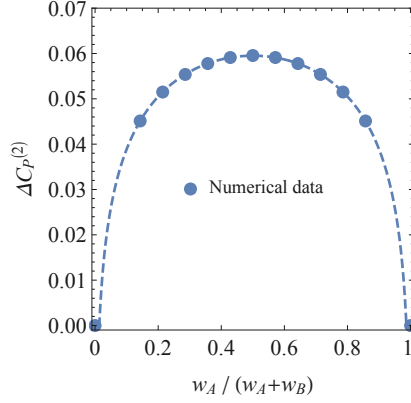
Figure 5.4.: Fermionic CoP for two adjacent ( d = 0 ) subsystems. The analytic form (5.33) is plotted as a dashed curve. Here we consider (w_A + w_B)/\delta = 14 sites for a total system size of N = 100(w_A + w_B)/\delta .
