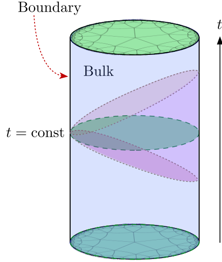
Figure 1.2.: Diagram of the bulk/boundary correspondence in AdS/CFT. The AdS_{D+1} spacetime is represented by the interior (bulk) of the cylinder, with its conformal boundary located represented by the boundary of said cylinder. A time slice t = \text{const} of AdS_{D+1} is a negatively-curved hyperbolic space. The pink shaded region corresponds to the Poincaré patch characterized by the metric (1.8).
