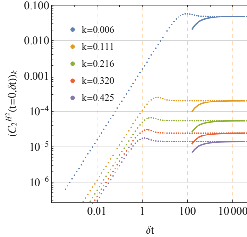
Figure 4.4.: Plot of single-mode contributions to C_2^{\mathbb{H}^2}(t=0, \delta t) as a function of \delta t for \omega_0 = 0.005 and for different values of k . The solid lines show an agreement of the exact (dotted) solutions with the saturation value (4.41) in the large \delta t KZ regime.
