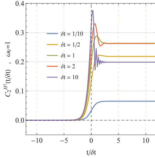
Figure 4.2.: Plot of \mathcal{C}_2^{\mathbb{H}^2}(t/\delta t) for \omega_0 = 1 and different values of \delta t . The oscillations observed for large \delta t arise from the rapidly oscillating behaviour of the solution (4.21) after passing through the critical point at t = 0 . Note the saturation of \mathcal{C}_2^{\mathbb{H}^2}(t/\delta t) for large t/\delta t , which is due to the choice of reference frequency \omega_0 = 1 .
