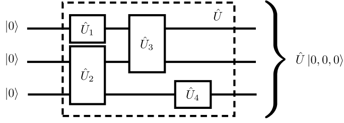
Figure 3.1.: A quantum circuit |\psi_T\rangle = \hat{U} |\psi_R\rangle = \hat{U} |0, 0, 0\rangle . The unitary \hat{U} is built from unitaries \hat{U}_i which act locally on the three qubits acting from left to right.
