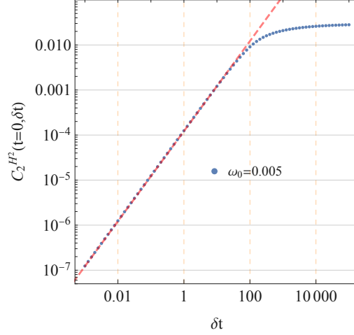
Figure 4.3.: Plot of \mathcal{C}_2^{H^2}(t=0, \delta t) as a function of \delta t for \omega_0 = 0.005 . The dashed red line shows a linear scaling \propto \delta t in the small \delta t regime.
