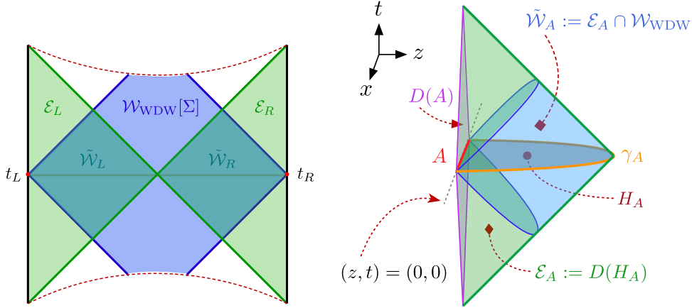
Figure 2.8.: Diagrams of the holographic subregion complexity proposals. On the left, a diagram of an eternal AdS black hole showing the entanglement wedges \mathcal{E}_{L,R} (shaded green regions) of the left and right CFTs, the Wheeler-De Witt (WDW) patch \mathcal{W}_{\text{WDW}} (shaded blue) and their intersections \tilde{\mathcal{W}}_{L,R} := \mathcal{E}_{L,R} \cap \mathcal{W}_{\text{WDW}} . On the right, a detail of one such intersections for a spatial subregion A on \text{AdS}_3 . The subregion CV proposal posits the equivalence of the complexity of the mixed state \rho_A defined on A to be given by the volume (area in this case) of H_A , \mathcal{C}_V \sim \text{Vol}(H_A) . The subregion CA and \text{CV}_{2,0} proposals posit instead that the complexity of \rho_A is given respectively by the evaluation of the gravitational action on, and by the spacetime volume of \tilde{\mathcal{W}}_A := \mathcal{E}_A \cap \mathcal{W}_{\text{WDW}} , namely \mathcal{C}_A \sim I_G[\tilde{\mathcal{W}}_A] and \mathcal{C}_{V_{2,0}} \sim \tilde{\text{Vol}}(\tilde{\mathcal{W}}_A) .
