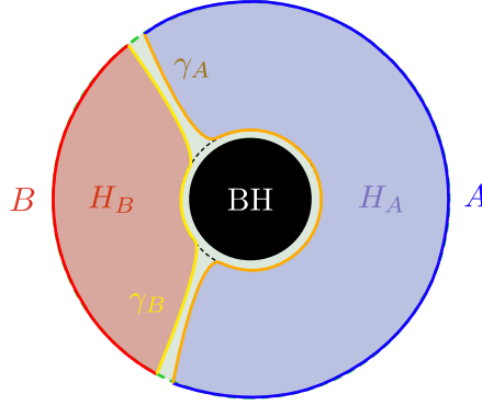
Figure 2.2.: Diagram of RT surfaces in the bulk of a time-slice of an \text{AdS}_3 Black Hole. The RT surfaces \gamma_A and \gamma_B associated with the boundary subregions A and B wrap around the black hole horizon, increasing their area as the size of the subregions increases. Note that the RT surfaces do not pierce through the horizon.
