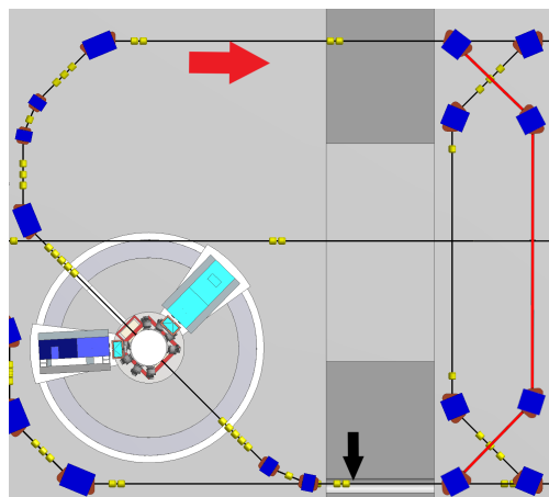
Figure 2: Top view of the planned recirculation line layout. The red line marks the beamline, that has to be built to close the ring, the black arrow marks the start of the simulation line and the red arrow marks the beam direction.
