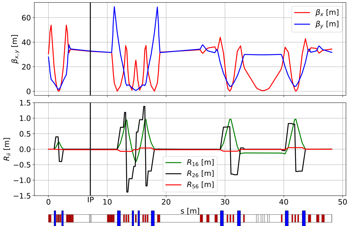
Figure 3: Simulations performed with MAD-X [7]. The layout below the graphs depicts the optical elements. Dipole magnets are blue and quadrupole magnets are red. The black line indicates the interaction point (IP) where the experiment is located.
