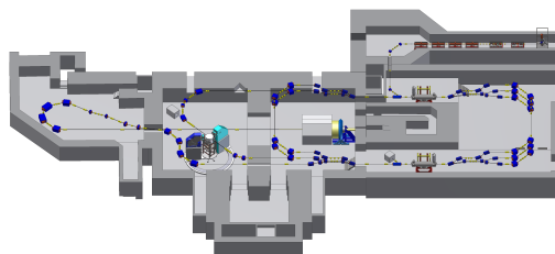
Figure 1: Rendering of the layout of the MESA facility. The injection beam line can be seen on the top right. The pseudo internal gas jet target is located in the fourth arc of the energy recovery mode.
