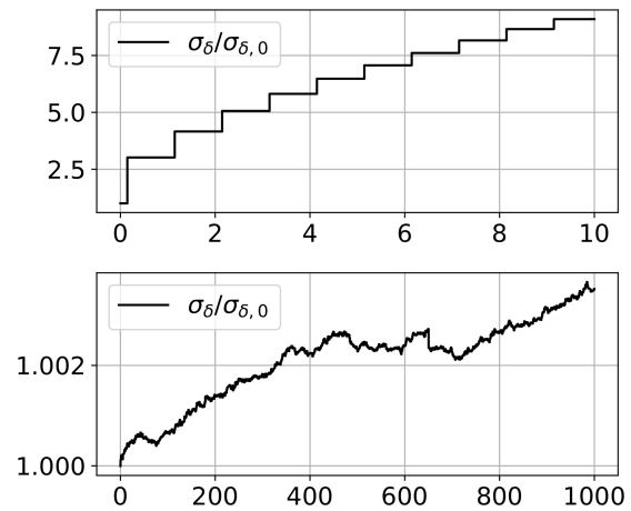
Figure 4: Comparison of the relative change in energy spread for the high density gas jet target simulated for 10 turns (top) with the scaled low density target simulated for 1 000 turns (bottom).
