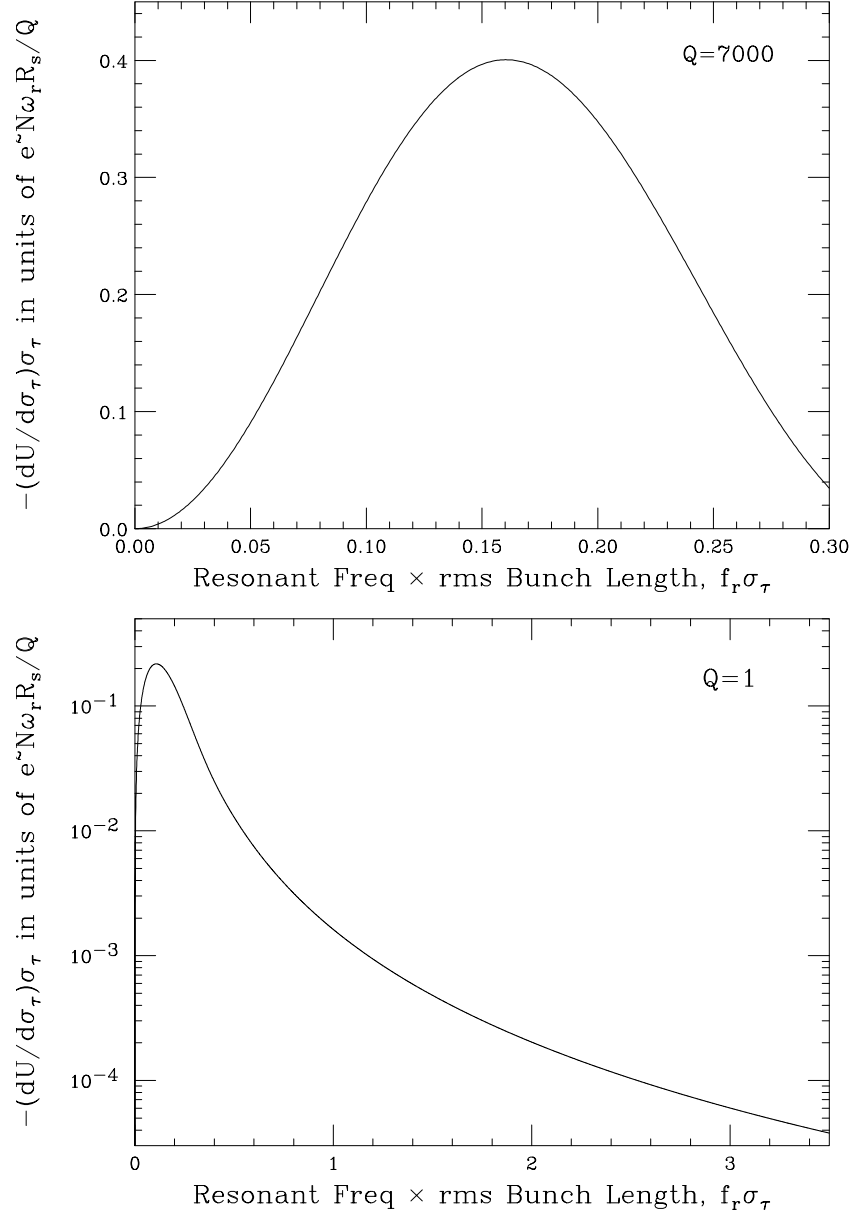
Figure 2: Plot of differential bunch energy loss (dU/d\sigma_\tau)\sigma_\tau versus f_r\sigma_\tau due to a sharp resonance (upper) or a broad-band impedance (lower).
