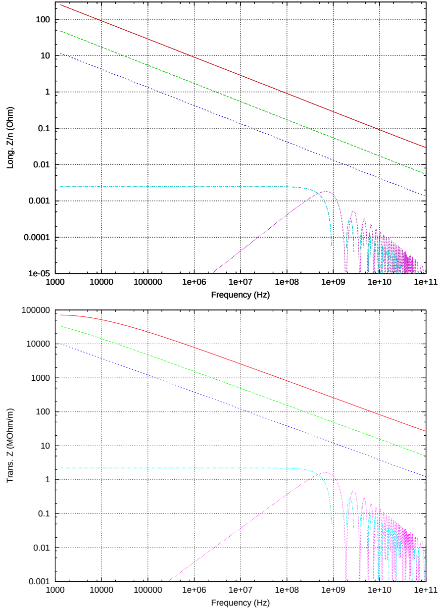
Figure 1: Longitudinal impedance Z_{\parallel}/n (upper plot) and transverse impedance (lower plot). In each plot, from top: real or imaginary parts of resistive wall contribution for a stainless steel beam pipe, an aluminum beam pipe, and a cold copper beam pipe. Lower curves: real and imaginary parts of the BPM contribution. All beam pipes are elliptical with radii 9 mm by 14 mm. One set of BPM striplines, either horizontal or vertical is assumed at each location of a FODO quadrupole. Each stripline is of length 8 cm subtending an angle of 30^\circ at the center of the pipe.
