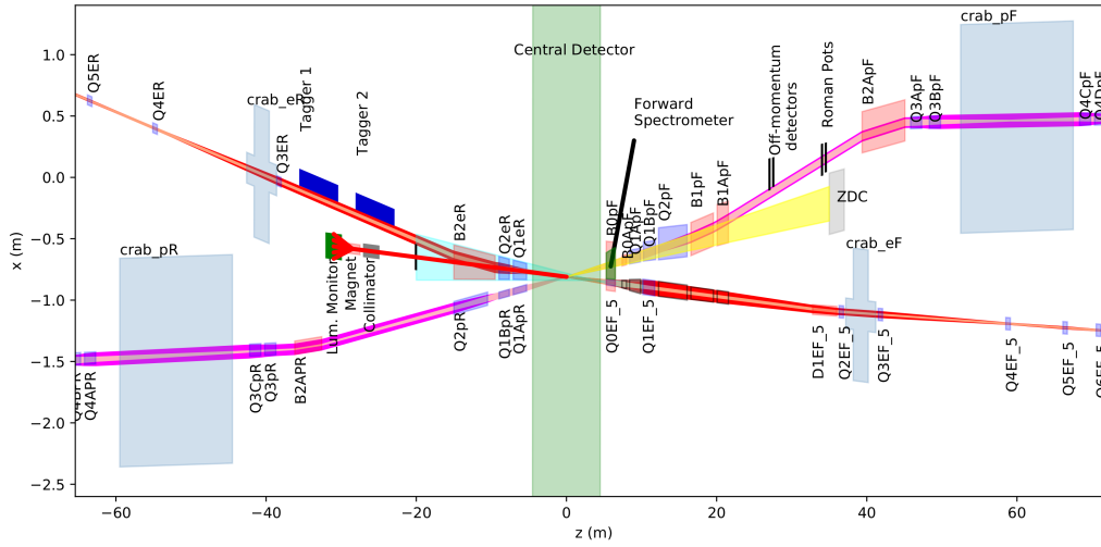
Figure 1: Layout of the interaction region of the EIC. In this figure the hadrons go from left to right. Shown in green is the central detector. Dipole and quadrupole magnet apertures are shown in pink and blue, respectively. Shown in grey are the crab cavities; the transverse size is illustrative of the size of the cavities. The neutron cone is shown in yellow and the synchrotron radiation fan in cyan.
