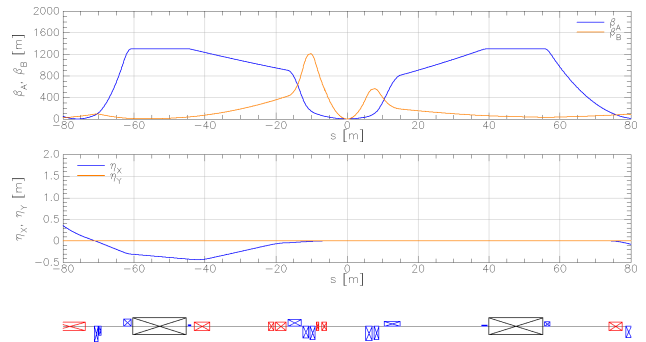
Figure 2: \beta function and dispersion of the hadron IR Lattice.
