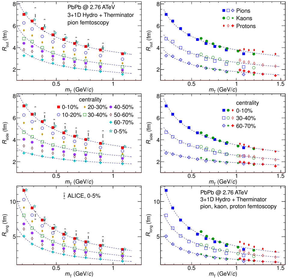
Fig. 2. (Left panel) Pion femtosopic radii from a hydrodynamic model of Pb–Pb collisions at the LHC, calculated as a function of pair transverse mass m_T = \sqrt{k_T^2 + m^2} and collision centrality. (Right panel) The radii for pions, kaons, and protons as function of pair transverse mass, for selected centralities. From [25].
