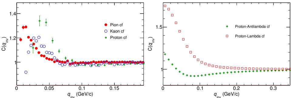
Fig. 1. Example correlation functions calculated in a model for central Pb–Pb collisions for pairs of identical pions, kaons, and protons (left panel) as well as for proton–lambda and proton–antilambda pairs (right panel).
