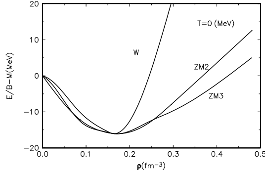
Fig. 2. The nucleon energy in function of nuclear matter density in the RMF approach for Walecka and ZM models [9].
