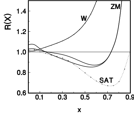
Fig. 3. Results for the ratio R(x) = F_2^{NM}(x)/F_2^N(x) which shows the evolution of the nucleon SF for Walecka (W) and ZM models of RMF for density \rho = 0.51 \text{ fm}^{-3} . Results for equilibrium density (SAT) \rho_0 = 0.17 \text{ fm}^{-3} the same for both models are shown for reference.
