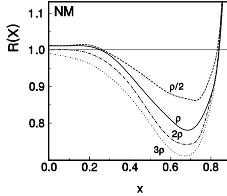
Fig. 4. Results for the ratio R(x) = F_2^{\text{NM}}(x)/F_2^{\text{N}}(x) which shows the evolution, without nuclear sea, of the nucleon SF for ZM2 model of RMF for densities \rho = \rho_0/2, \rho_0, 2\rho_0, 3\rho_0 . \rho_0 = 0.16 \text{ fm}^{-3} is the equilibrium density for NM.
