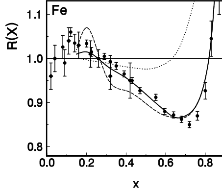
Fig. 1. Ratio of the nuclear (iron) SF F_2(x) to deuterium in the deep inelastic electron–nucleus scattering.
