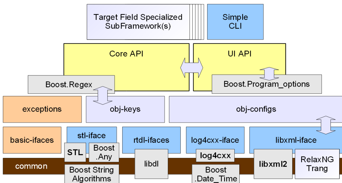
Figure 1. Project architecture layout (the dependent external software packages and the most important dependencies between the layers of hierarchy are also shown). “Target Filed Specialized SubFrameworks” on the top of the structure are to be implemented by the users.
