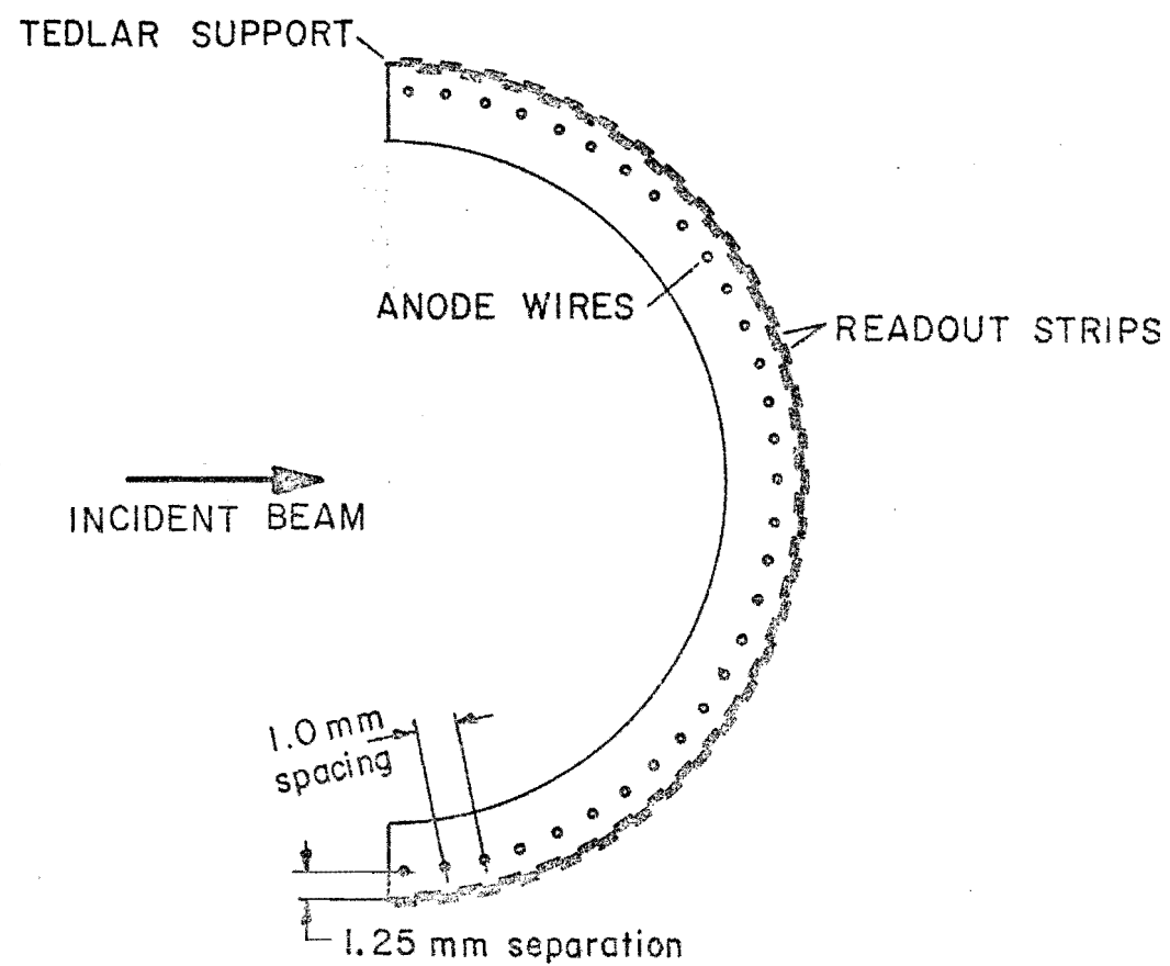
CYLINDRICAL PROPORTIONAL CHAMBER
