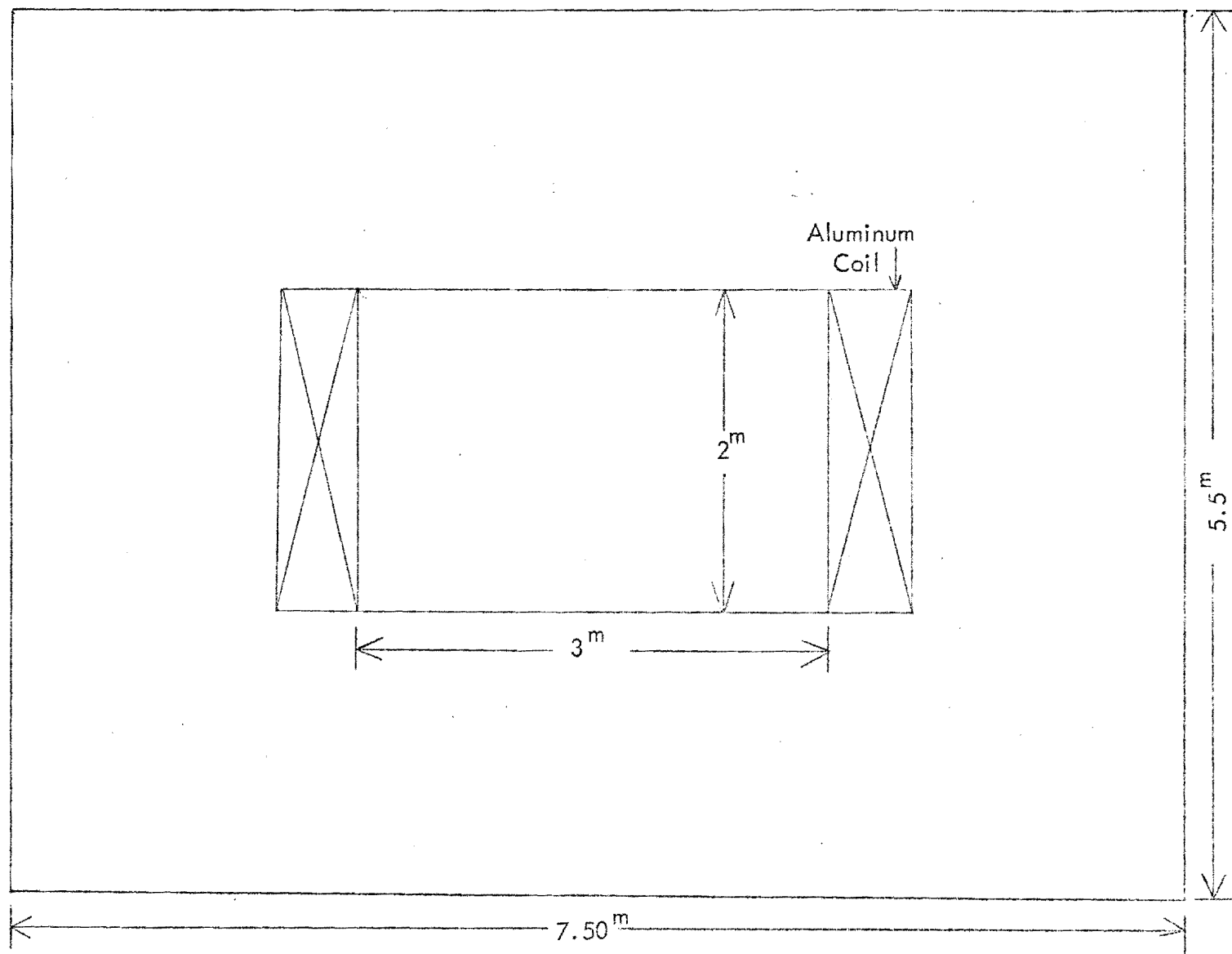
Figure 12. Cross section of the 6 meter long picture frame bending magnet.
