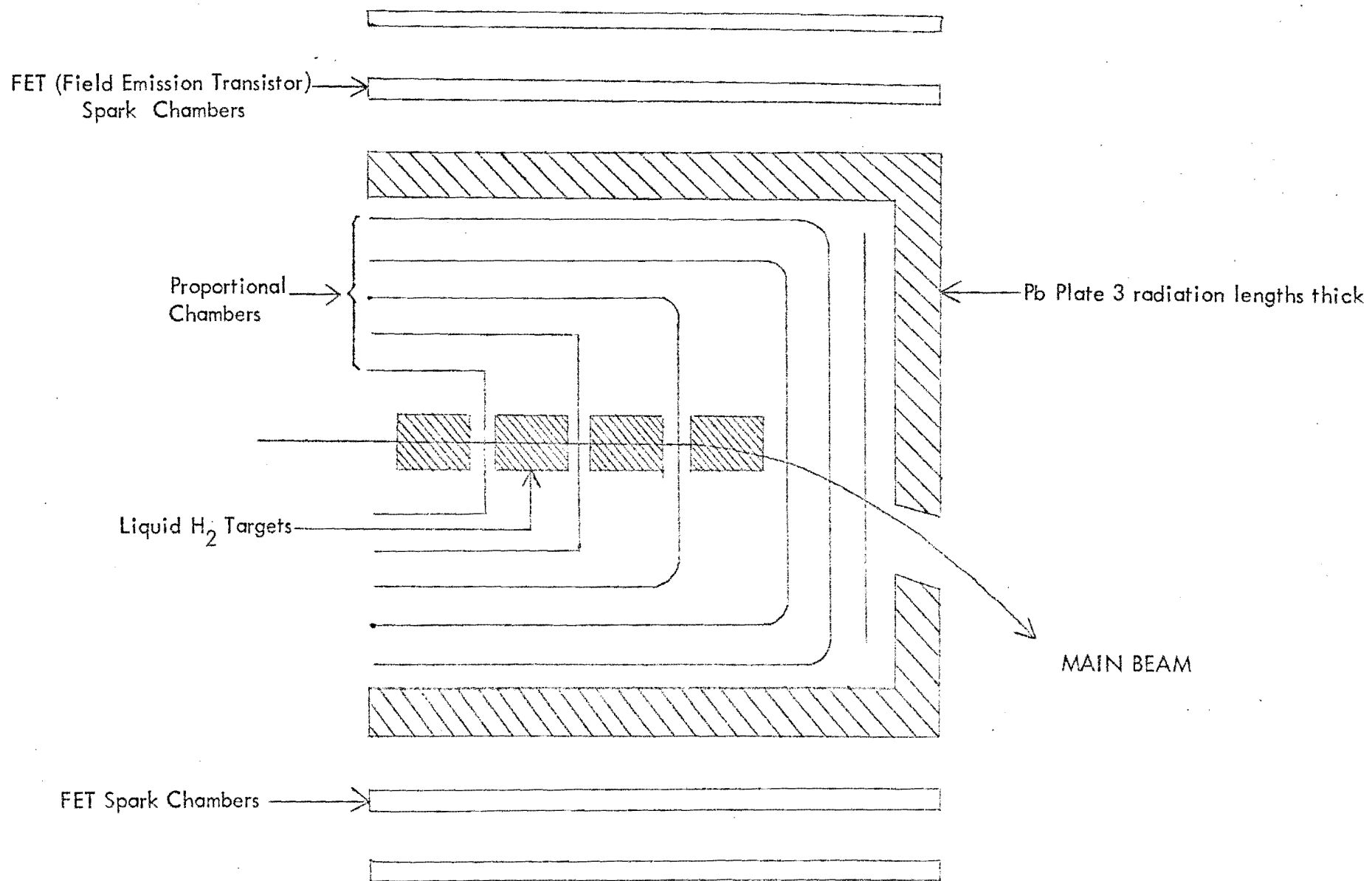
Figure 10b. Target Setup (Not to Scale)
