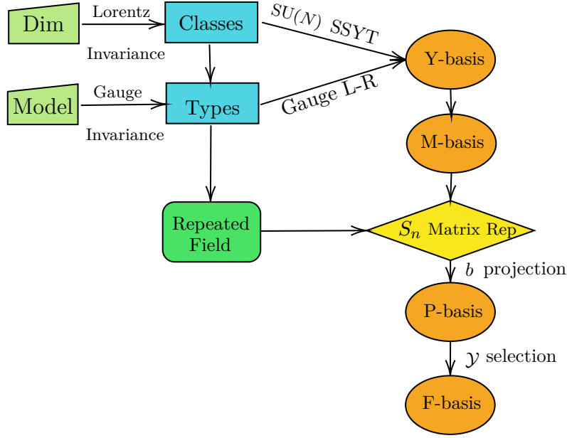
Figure 1. Flow chart of the ABC4EFT package for finding all independent operators for a given model at certain mass dimension. The Lorentz Y-basis is constructed using semi-standard Young tableaux (SSYTs) and the gauge Y-basis is constructed using Littlewood-Richardson rules. To deal with repeated fields, we introduce the matrix representation of the generators of the symmetric group S_n , and construct the matrix representation of the projection operator b to get the p-basis. Finally we select the first projection operators b of each S_n representation, which correspond to Young symmetrizers \mathcal{Y} , and obtain the flavor-specified operators as the f-basis.
