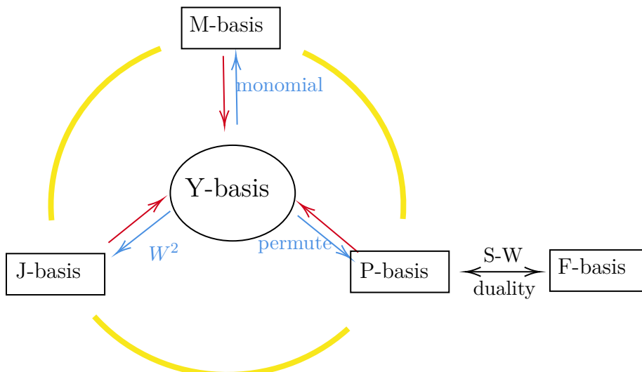
Figure 2. Relations among the bases. The red arrow means that the basis can always be able to find its coordinates on the y-basis through a reduce procedure. The yellow circle indicates that the m-basis, p-basis and j-basis are related by linear transformations. The operators in the p-basis are tensors of the symmetric group S_m , and these in f-basis are tensors of SU(n_f) group, where m is the number of repeated fields and n_f is the flavor number of each repeated field. These two basis are connected by the Schur-Weyl duality.
