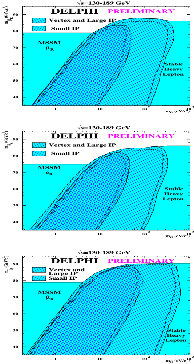
Figure 8: Exclusion regions in the (m_{\tilde{G}}, m_{\tilde{\mu}_R}) (upper plot), (m_{\tilde{G}}, m_{\tilde{e}_R}) (middle plot) and (m_{\tilde{G}}, m_{\tilde{l}_R}) (bottom plot) planes at 95% C.L. for the present analysis combined with the stable heavy lepton search and the MSSM \tilde{\tau}_R search, using all LEP-2 data. The positive-slope hatched area shows the region excluded by the small impact parameter search. The negative-slope hatched area shows the region excluded by the combination of the large impact parameter and secondary vertex searches. The dashed line shows the expected limits. For \tilde{e}_R only the contribution of s -channel has been considered.
