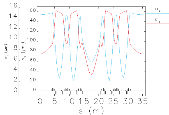
Figure 4: The beam envelope in a super period of the ILSF ring, second lattice option.
