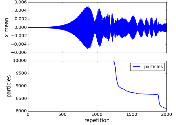
Figure 4: The centroid position of a bunch operating in anti-damper with the gain set to -0.01 and the number of macro-particles using the full nonlinear propagation of drifts.
