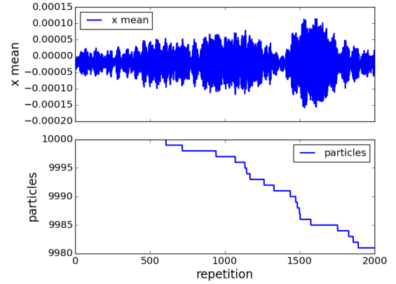
Figure 5: The centroid position of a bunch and the number of macro-particles operating in anti-damper mode with the gain set to -0.01 using the full nonlinear propagation of drifts with an integrable nonlinear element.
