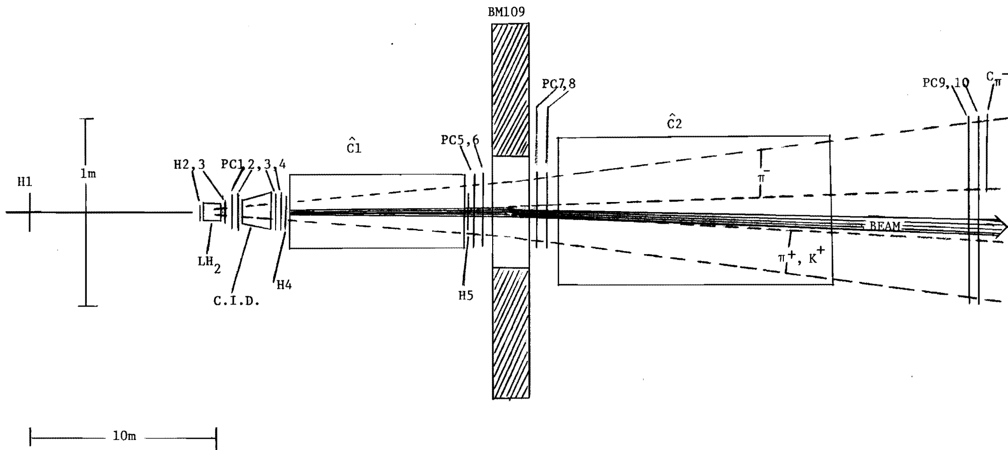
FIGURE 2 Proposed Layout of Apparatus
