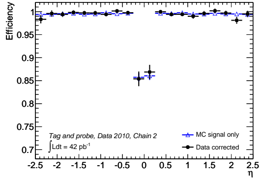
(f) Muid efficiency as a function of \eta(\mu)
