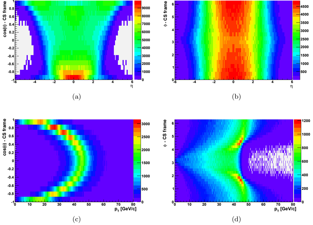
Figure 7.2.: Correlations between the decay angles \cos\theta (left) / \phi (right) and the kinematic properties of the decay muon \eta (upper row) / p_T (lower row).
