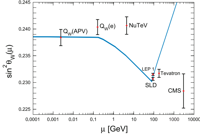
Figure 2.3.: Scale dependence of the weak mixing angle defined in the \overline{\text{MS}} scheme [17].
