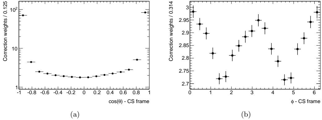
Figure 7.8.: Weights to correct the influence of the detector on the angular distributions in the range 15 \text{ GeV}/c < p_T(\mu\mu) < 20 \text{ GeV}/c . In particular, the \cos \theta spectrum (a) is affected by the limited acceptance of the detector. Correction factors on the \phi spectrum show lower fluctuations and reflect the overall acceptance of about 37%.
