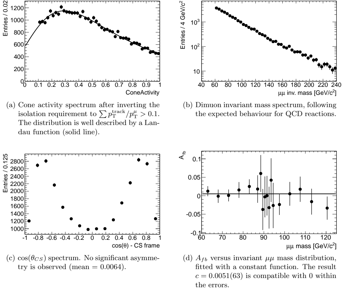
Figure 6.14.: Spectra of QCD events selected from the data sample by inverting the isolation requirement.
