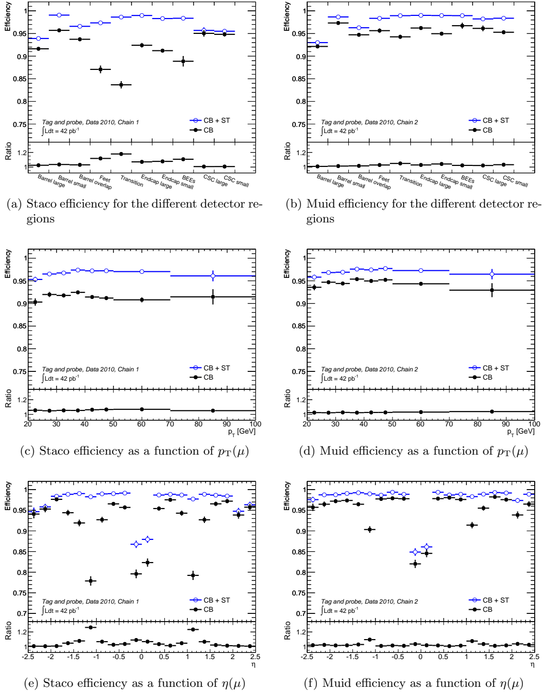
Figure 5.4.: Efficiencies for combined plus segment-tagged muons (open circles) in comparison to those for combined muons only (dots) for the two reconstruction chains Staco (left) and Muid (right). The relative gain is shown in the lower part of each figure.
