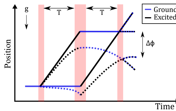
Figure 1. The atom interferometry sequence: As the atoms fall under the effect of gravity, a laser pulse is used to put them into a quantum superposition of the ground and excited states. The action of this pulse can be thought of as sending each atom along two simultaneous but different paths in the gravity field (as a consequence of wave-particle duality). After a time, T , a second laser pulse is then used to cause the paths to converge again at time 2T . At this time, the atoms are recombined using a final laser pulse; the final state of the atoms encodes the value of gravity. Dotted and solid lines show the sequence with and without gravity, respectively, where the deflection due to gravity introduces a phase shift \Delta\phi to the interferometer.
