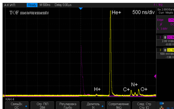
Fig. 4: TOF spectrum obtained at the test bench for the helium ion source.
