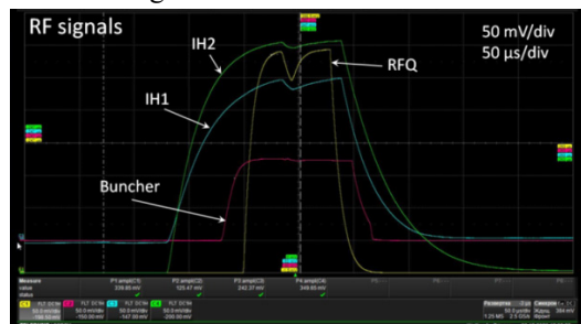
Fig. 10: RF dropdowns in the HILAC cavities.
