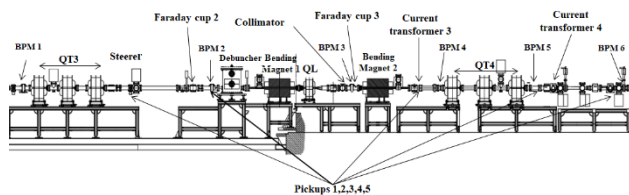
Fig. 8: Beam diagnostic units arranged along HEBT.
