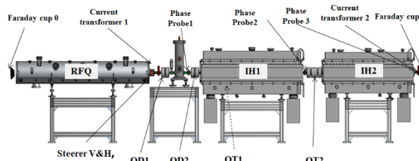
Fig. 7: Beam diagnostic units arranged along HILAC.
