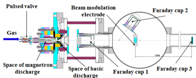
Figure 2: Test bench layout for the TOF measurements.
