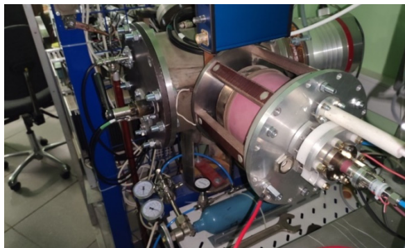
Figure 3: Helium ion source at the test bench.
