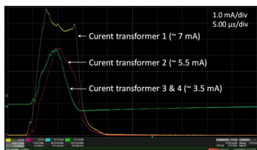
Fig. 9: Current transformer signals, 7 mA-RFQ output, 5.5 mA-IH2 output, 3.5 mA –behind QT4 triplet.
