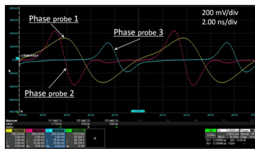
Figure 12: Phase probe signals produced helium beam, 1-behind RFQ, 2-behind IH1, 3-behind IH3.
