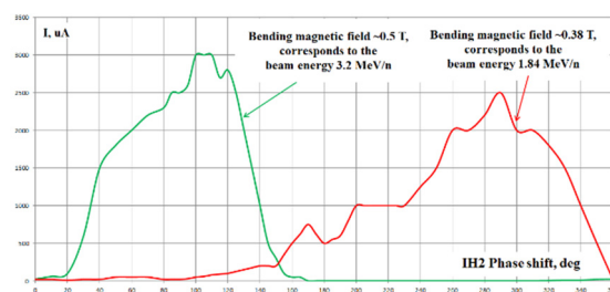
Figure 11: Faraday cup 3 signal vs RF phase shift of IH2.
