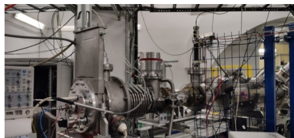
Figure 5: Helium ion source on the HV terminal fixed to the LEBT
