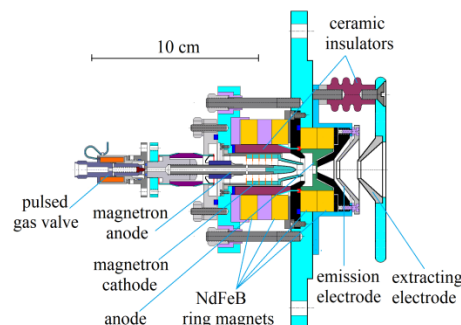
Fig. 1 Helium ion source design.
