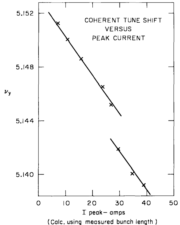
FIG. 3--Measured vertical betatron tune versus peak circulating current.
