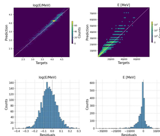
Figure 5. Output of the \log(E/MeV) network and the respective results for the true value of the energy (in MeV ). The plots show the correlation between targets and predictions (above) and the residuals (below).
