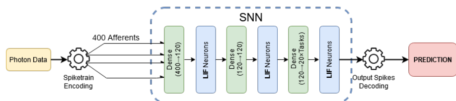
Figure 4. Data processing pipeline and network architecture.
