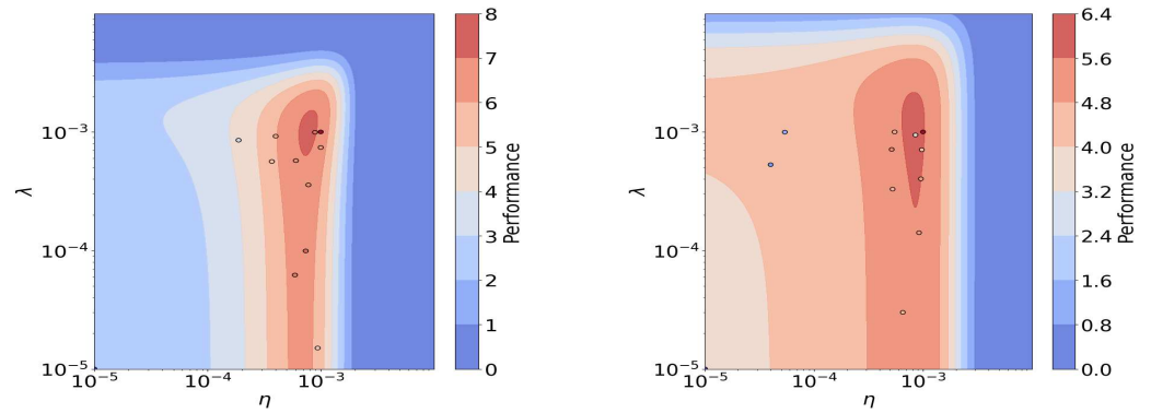
Figure 11. Posterior distribution of network performance on \log(E/MeV) and centroid (left) and \log(E/MeV) and dispersion (right) for multi-target regression learning rate \eta and weight regularization constant \lambda , having set the number of layers to N = 2 and the network width to W = 120 , as obtained from the architecture optimization above.
