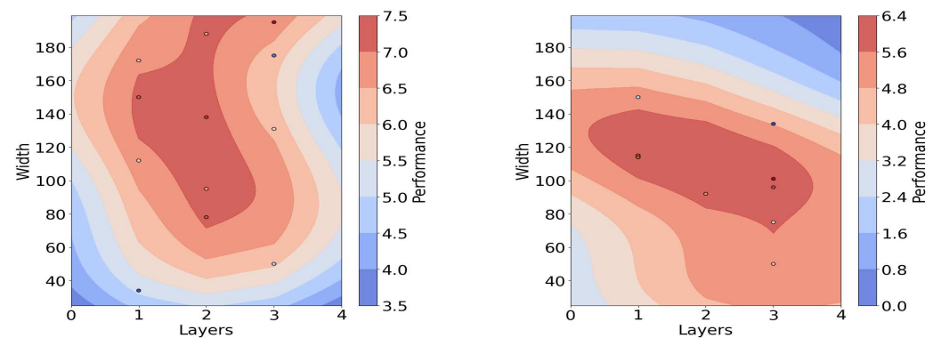
Figure 10. Posterior distribution of network performance on \log(E/\text{MeV}) and centroid (left) and \log(E/\text{MeV}) and dispersion (right) for multi-target regression as a function of the layers and width per layer, having set \eta = 10^{-4} and \lambda = 0 .
