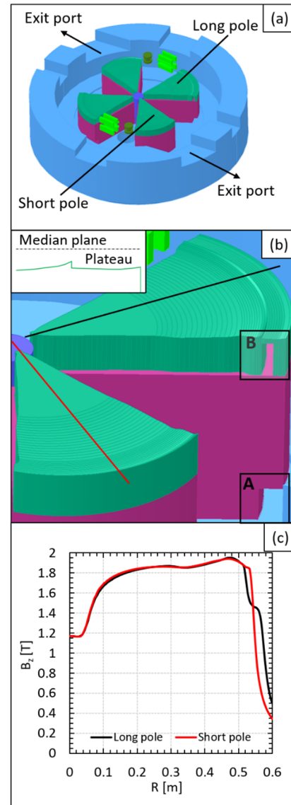
Figure 2: (a) 3D FE model of the cyclotron iron; (b) 3D design of the long pole; (c) Magnetic field along a line that bisects the long and short poles, as shown in (b).
