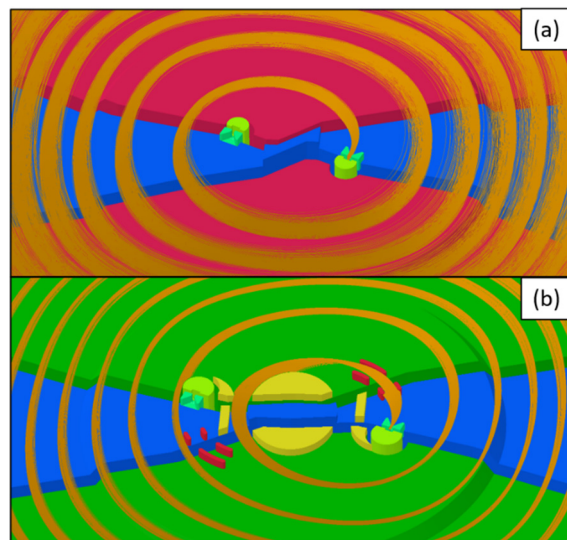
Figure 4: (a) A simulated well-centered beam in the 3D cyclotron central region model; (b) A simulated beam with a large orbit centering error in the 3D cyclotron central region model with the off-centered ion sources.
