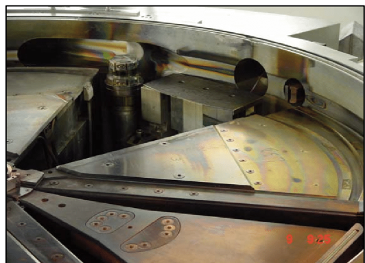
Figure 1: The groove in the long pole, the gradient corrector and the beam separator in the prototype.
