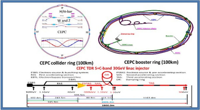
Figure 1. CEPC-SppC layout.
