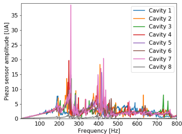
Figure 7: Main mechanical modes for all eight cavities of XM50.1, measured using a frequency sweep piezo excitation.
