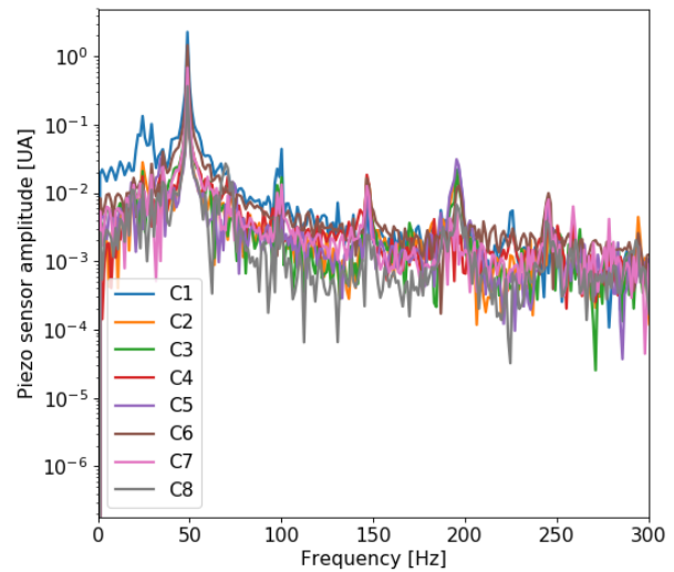
Figure 5: Background microphonics measured with piezos installed on all eight cavities of XM50.1, once installed at CMTB.
