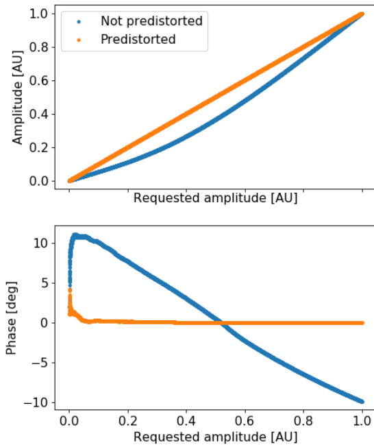
Figure 4: IOT amplitude (top) and phase (bottom) linearized using the pre-distortion module in the LLRF main controller firmware.
