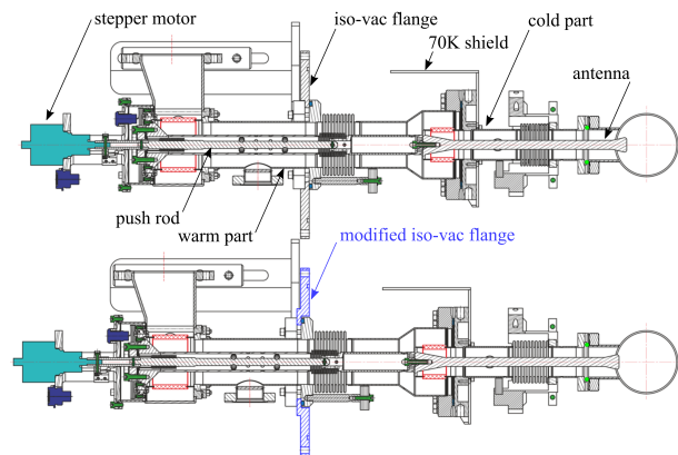
Figure 1: Unmodified XFEL power coupler (top) and with the modified iso-vac flange (bottom), shifting outwards the warm part of the coupler.
