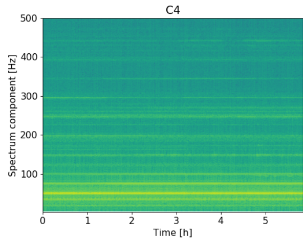
Figure 6: Long term measurement of the background microphonics spectrum of XM50.1 cavity 4.
