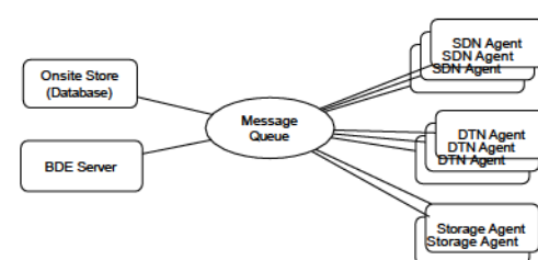
Message-Queue-based Framework
