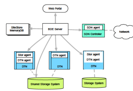
BigData Express Architecture (II)
