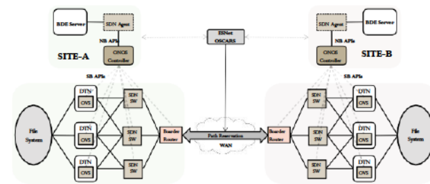
End-to-End Network Path
