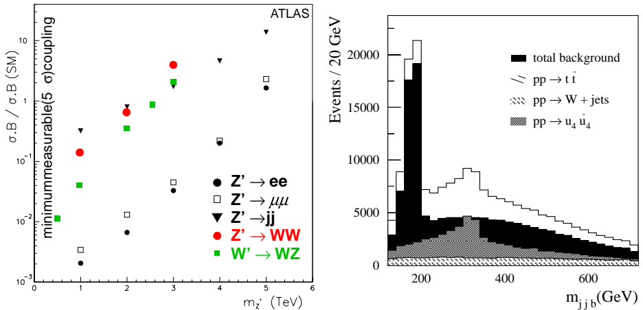
Fig. 4. (Left) Limits ( 5\sigma ) on W' and Z' coupling for fermionic ( 100\text{ fb}^{-1} ) and bosonic ( 300\text{ fb}^{-1} ) decay modes [1]. (Right) Invariant mass distribution for 320\text{ GeV} forth generation quark u_4 \rightarrow bW \rightarrow bjj [1].
