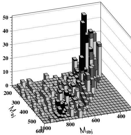
Fig. 7. Mass distribution for \pi_T^\pm of 300 GeV and \rho_T^\pm of 500 GeV in \rho_T^\pm \rightarrow \pi_T^\pm Z \rightarrow bq \ell^+ \ell^- ( 30\text{fb}^{-1} ) [1]. Signal in black, t\bar{t} background in dark gray, Zj — light gray.
