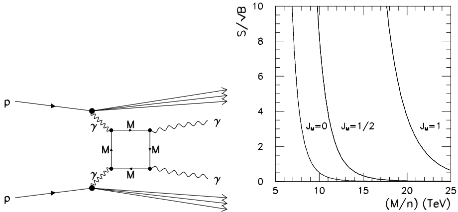
Fig. 5. (Left) Monopole production at LHC. (Right) Significance contours for monopoles of spin J_M , mass M and charge n ( 100\text{ fb}^{-1} ) [1].
