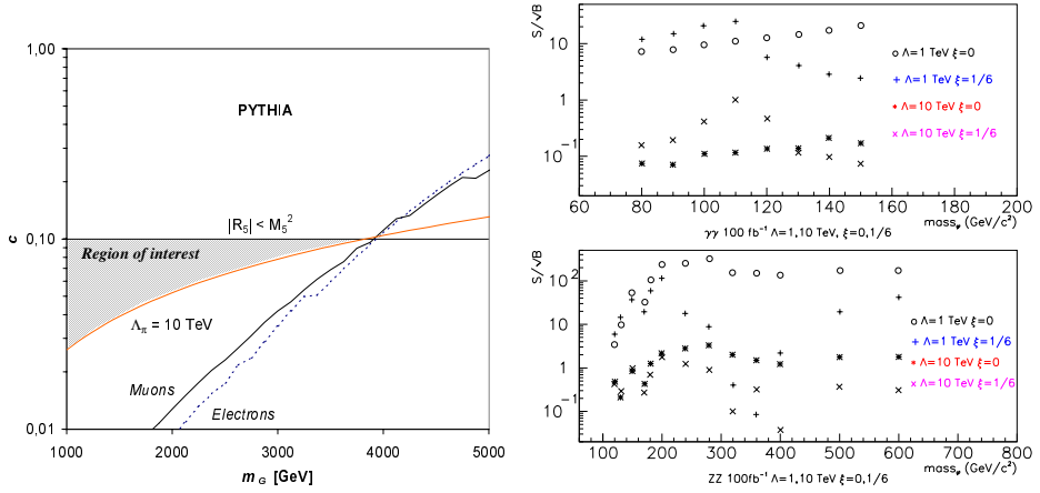
Fig. 8. (Left) Search for RS graviton G \rightarrow \ell\ell . Couplings c > 0.01 – 0.1 are accessible for masses m_G > 2 – 4 TeV respectively [8]. (Right) Significance for radion signal in \phi \rightarrow \gamma\gamma (upper plot) and \phi \rightarrow ZZ (lower plot) channels [9].
