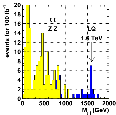
Fig. 6. Mass distribution for scalar, 2 nd generation leptoquarks of 1.6 TeV produced in pairs [6].
