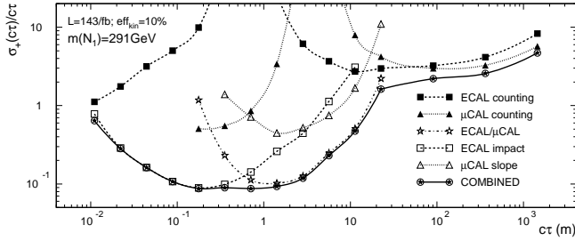
Fig. 3. Relative precision of neutralino lifetime measurement [5].
