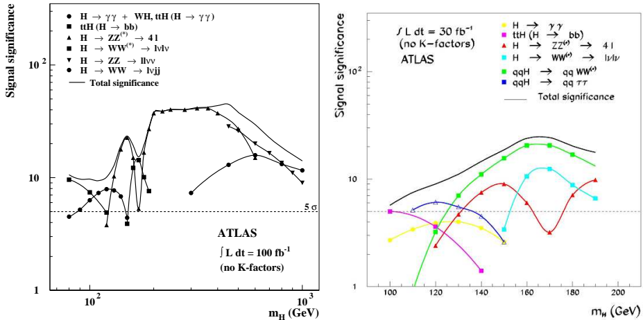
Fig. 1. (Left) SM Higgs search in various channels [1]. (Right) Low mass SM Higgs search in vector boson fusion channels [3].
