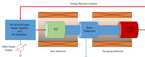
Figure 5: Schematic overview of the electron gun test bench.
