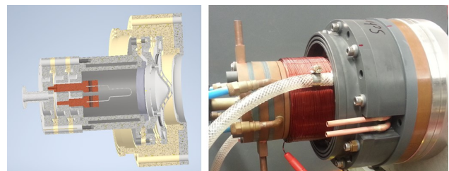
Figure 2: Technical drawing (left) and actual electron gun (right).
