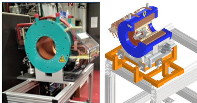
Figure 3: Picture of gun solenoid (left) and technical drawing of integrated electron gun set-up (right).
