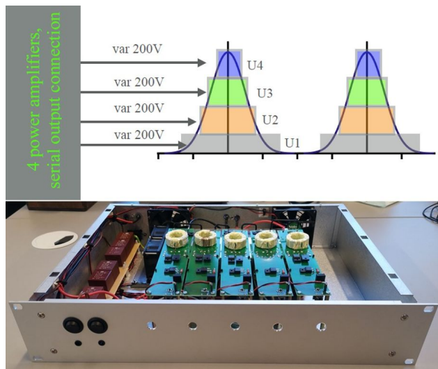
Figure 4: Working principle of multi-level inverter and picture of scaled (4-level) power modulator.
