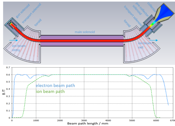
Figure 1: The SCC electron lens magnet system and the absolute value of magnetic field on the ion beam and the electron beam orbit.
