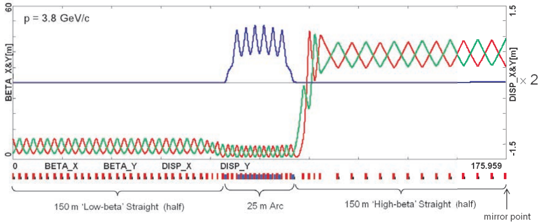
Figure 12. Complete racetrack ring lattice. Only half of the ring is shown, with the mirror symmetry point indicated on the right end.
