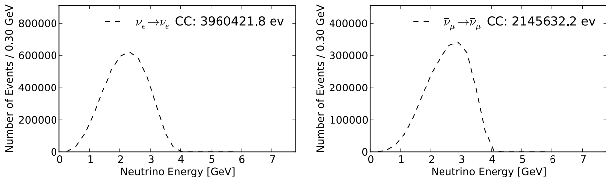
Figure 39. \nu_e spectrum at near detector (Left), \bar{\nu}_\mu (Right).
