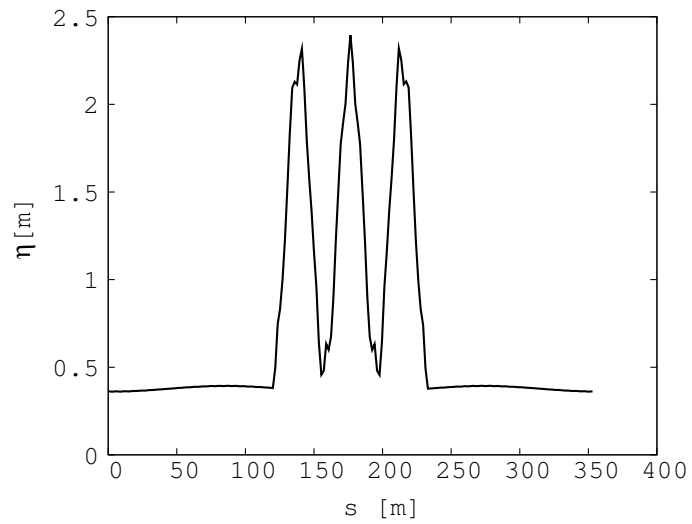
Figure 23. Dispersion function for p_0 in half of the ring. The plot is centered on the arc part.
