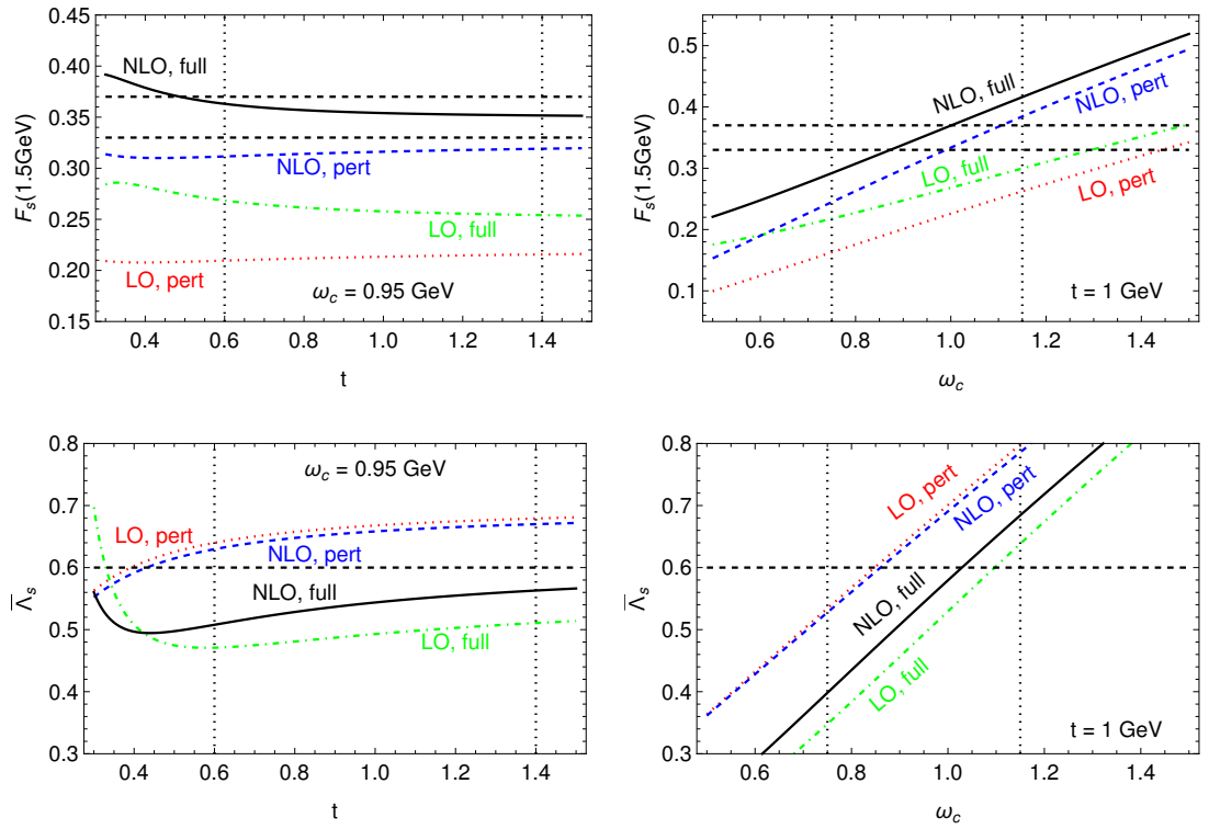
Figure B.3: Dependence of the sum rule results for F_s(\mu) (top) and \bar{\Lambda}_s (bottom) on the Borel parameter t (left) and the continuum cutoff \omega_c (right) in the B_s system.
