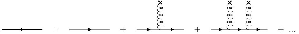
Figure 2.7: Vacuum gluon corrections to the quark propagator.
