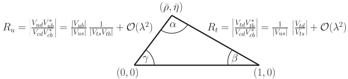
Figure 4.1: Our conventions for the unitarity triangle in the \bar{\rho} - \bar{\eta} plane.
