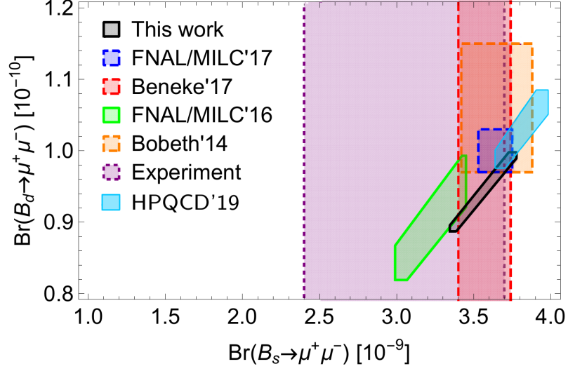
Figure 3.5: We compare our prediction for the branching ratios \mathcal{B}(B_q^0 \rightarrow \mu^+ \mu^-) with q = s, d to other predictions using either the decay constants [160, 174, 176] (dashed boundaries) or the Bag parameter \overline{B}_{Q_1}^q [137, 156] (solid boundaries) as input. The experimental average for \mathcal{B}(B_s^0 \rightarrow \mu^+ \mu^-) is indicated by the region with the dotted boundary.
