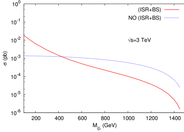
Fig. 3. Cross sections for e^-e^+ \rightarrow \tilde{\nu}_\tau \tilde{\nu}_\tau^* process at CLIC with \sqrt{s} = 3 TeV.
