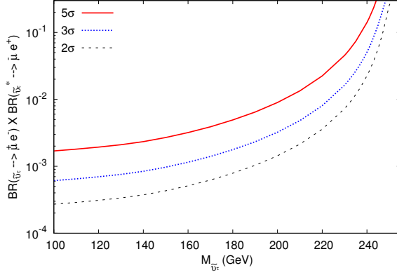
Fig. 4. Achievable limits for \text{Br}(\tilde{\nu}_\tau \rightarrow \mu^+ e^-) \times \text{Br}(\tilde{\nu}_\tau^* \rightarrow \mu^- e^+) versus tau-sneutrino mass values at CLIC with \sqrt{s} = 0.5 TeV.
