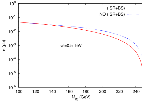
Fig. 2. Cross sections for e^-e^+ \rightarrow \tilde{\nu}_\tau \tilde{\nu}_\tau^* process at CLIC with \sqrt{s} = 0.5 TeV.
