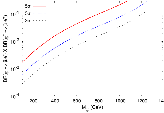
Fig. 5. Achievable limits for \text{Br}(\tilde{\nu}_\tau \rightarrow \mu^+ e^-) \times \text{Br}(\tilde{\nu}_\tau^* \rightarrow \mu^- e^+) versus tau-sneutrino mass values at CLIC with \sqrt{s} = 3 TeV.
