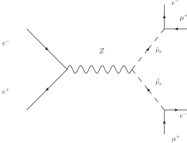
Fig. 1. Feynman diagram for e^+e^- \rightarrow \tilde{\nu}_\tau \tilde{\nu}_\tau \rightarrow \mu^+e^- \mu^+e^- process.
