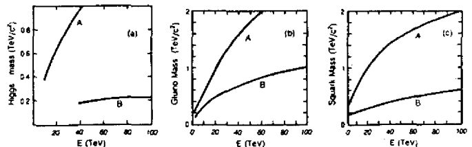
Fig. 1. (a) H \rightarrow W^+W^- . The SSC (curve A at 40 TeV cm) can plausibly discover any Higgs particle with a mass between 0.2 and 1.0 TeV. The lower-luminosity collider has a very narrow window for discovery of a heavy Higgs via the W^+W^- decay mode.
