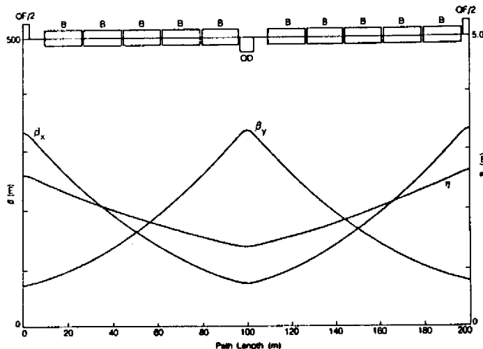
Fig. 2. The betatron amplitude functions ( B_x, B_y ) and the dispersion function ( \eta ) in the regular cells for the high field lattice.
