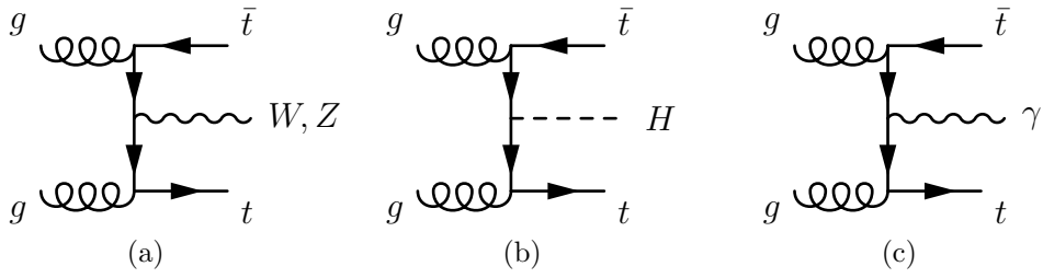
FIGURE 5. Top quark production in association with a boson
