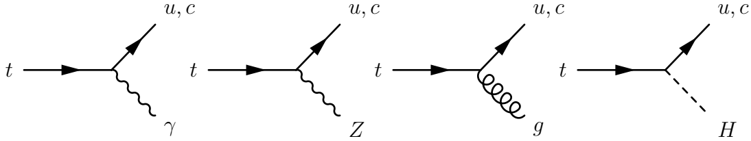
FIGURE 10. Flavor-changing neutral top quark decays (forbidden at tree-level)
