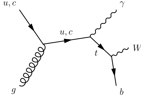
FIGURE 14. FCNC search by CMS in single top production
