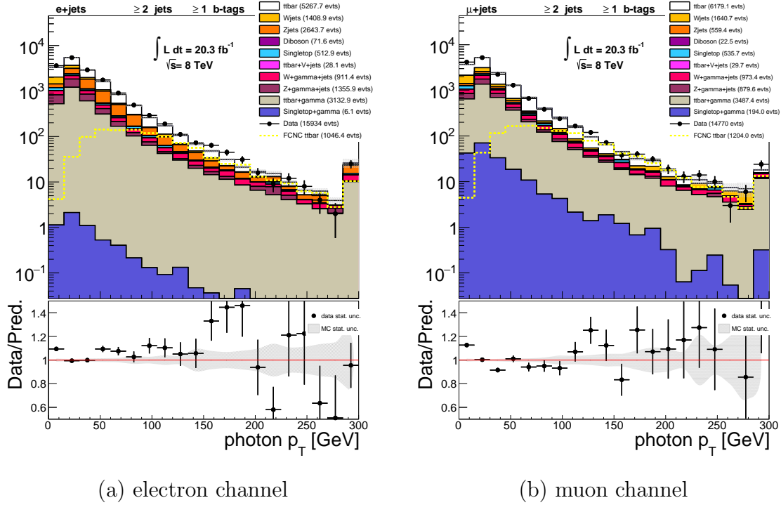
FIGURE 38. Photon candidate p_T after the signal region pre-selection, in the electron and muon channels. FCNC signal BR(t \rightarrow q\gamma) is scaled to 1% on these plots. A photon candidate p_T cut of 50 GeV is applied to the final signal selection.
