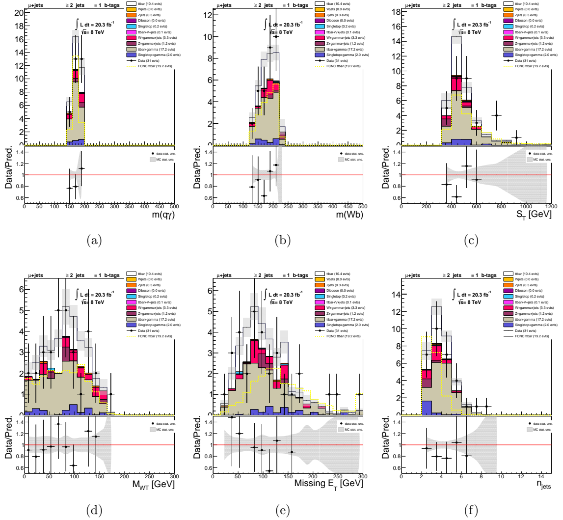
FIGURE 65. FCNC top mass (a), SM top mass (b), S_T (c), m_T^W (d), E_T^{\text{miss}} (e), and N_{\text{jets}} (f) plots in the signal region, with scale factors applied (muon channel)
