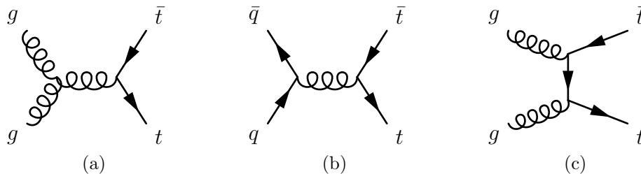
FIGURE 3. Top quark pair production mechanisms
