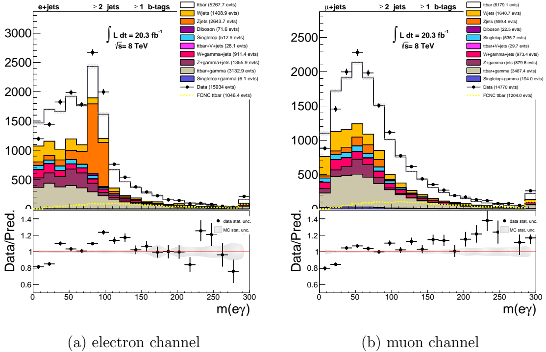
FIGURE 43. Invariant mass of the electron and photon candidates, m(e\gamma) , after the signal region pre-selection, in the electron and muon channels. FCNC signal \text{BR}(t \rightarrow q\gamma) is scaled to 1% on these plots. A cut of |m(e\gamma) - m_Z| > 5 \text{ GeV} is applied to the final signal selection.
