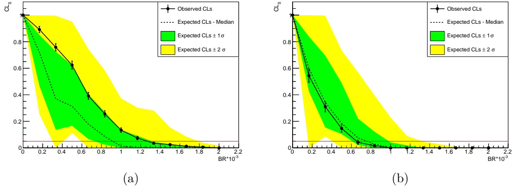
FIGURE 66. Expected and observed upper limits on the branching ratio \text{BR}(t \rightarrow q\gamma) for the electron (a) and muon (b) channels
