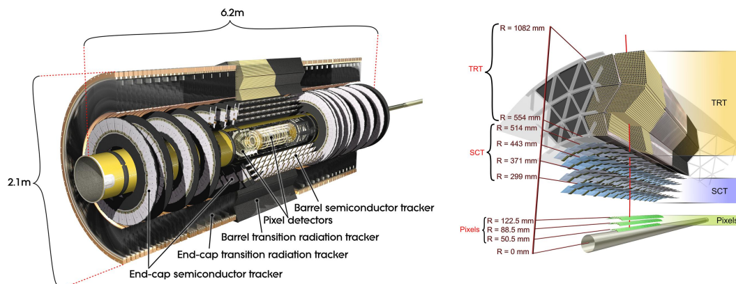
FIGURE 24. The ATLAS inner detector [39]
