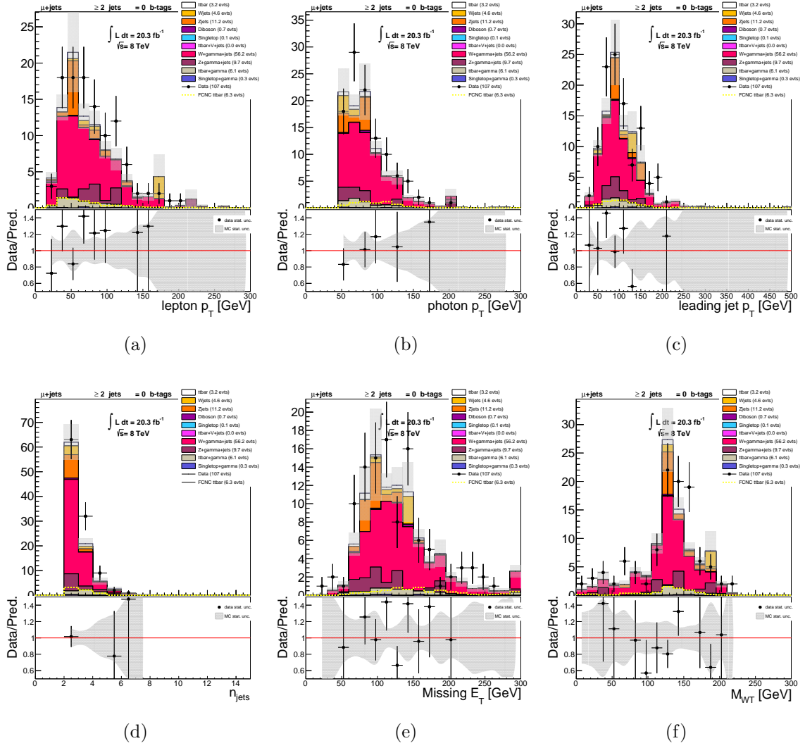
FIGURE 49. Lepton p_T (a), photon p_T (b), leading jet p_T (c), N_{jets} (d), E_T^{miss} (e), and m_T^W (f) distributions for the W+\gamma validation region (muon channel). FCNC signal BR( t \rightarrow q\gamma ) is scaled to 0.1%
