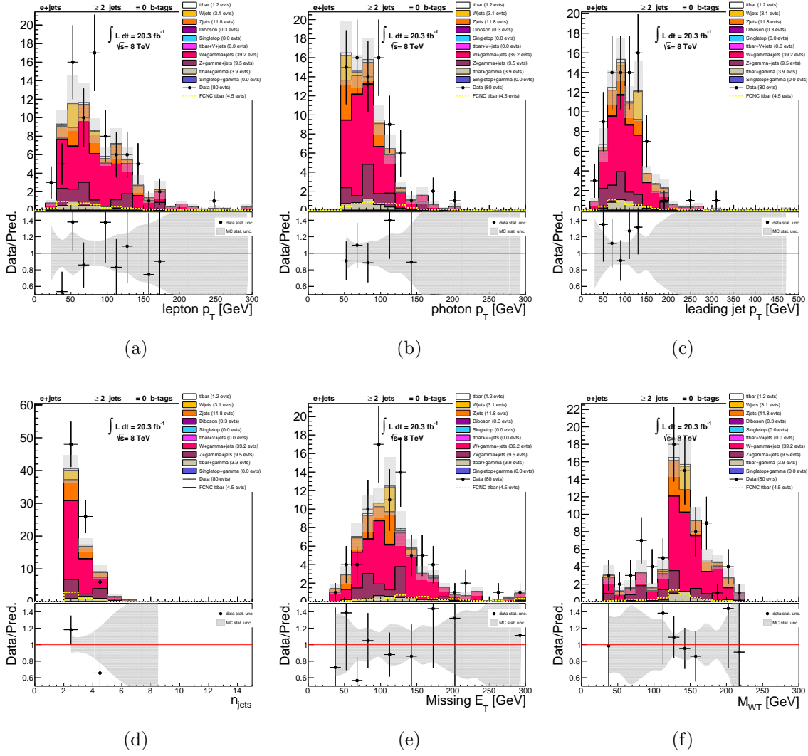
FIGURE 48. Lepton p_T (a), photon p_T (b), leading jet p_T (c), N_{jets} (d), E_T^{\text{miss}} (e), and m_T^W (f) distributions for the W+\gamma validation region (electron channel). FCNC signal \text{BR}(t \rightarrow q\gamma) is scaled to 0.1%
