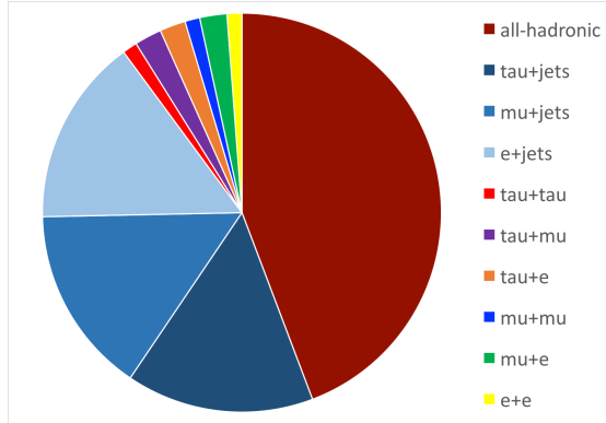
FIGURE 7. Top quark decays in the SM can be further categorized by the decay of the W boson
