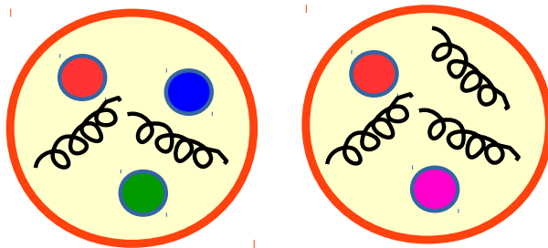
FIGURE 2. Artist's rendition of a baryon ( qqq ) and a meson ( q\bar{q} )
