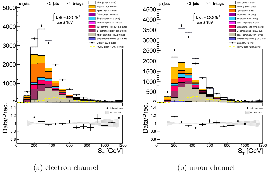
FIGURE 44. S_T after the signal region pre-selection, in the electron and muon channels. FCNC signal \text{BR}(t \rightarrow q\gamma) is scaled to 1% on these plots. A cut of S_T > 375 GeV is applied to the final signal selection.
