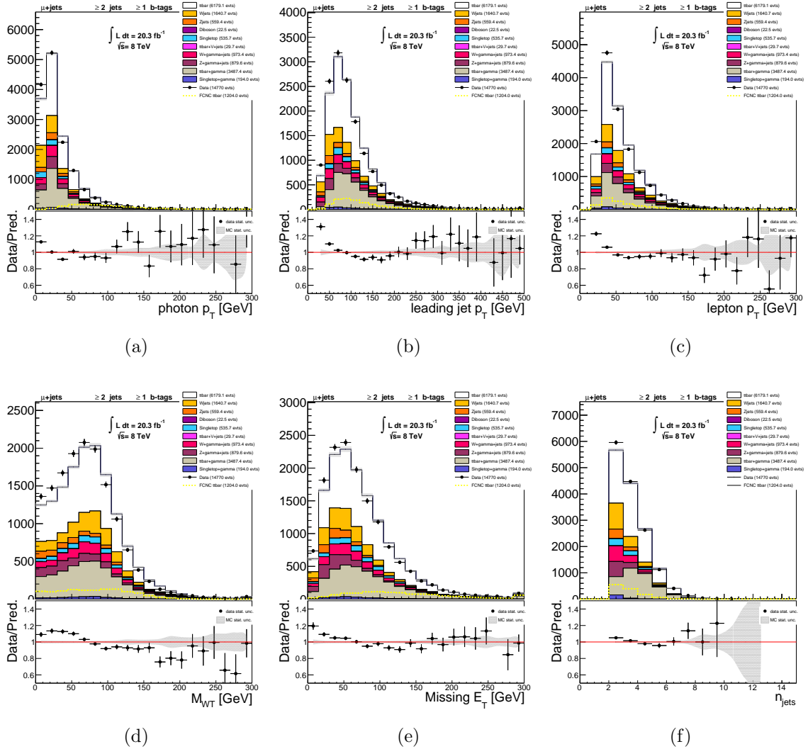
FIGURE 47. Photon p_T (a), leading jet p_T (b), lepton p_T (c), m_T^W (d), E_T^{\text{miss}} (e), and N_{jets} (f) plots in the signal pre-selection region (muon channel)
