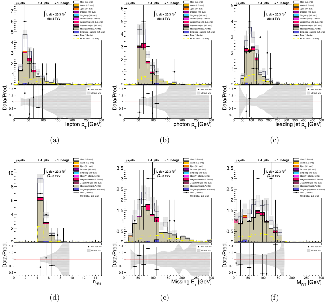
FIGURE 51. Lepton p_T (a), photon p_T (b), leading jet p_T (c), N_{jets} (d), E_T^{\text{miss}} (e), and m_T^W (f) distributions in the t\bar{t} + \gamma validation region (muon channel). FCNC signal \text{BR}(t \rightarrow q\gamma) is scaled to 0.1%.
