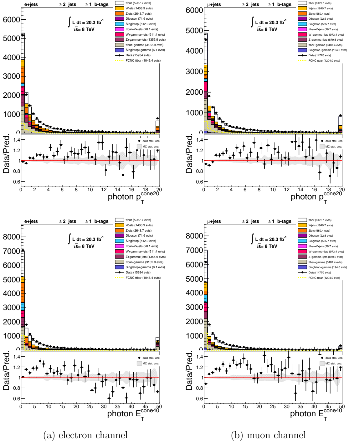
FIGURE 39. Photon isolation variables, after the signal region pre-selection, in the electron and muon channels. FCNC signal \text{BR}(t \rightarrow q\gamma) is scaled to 1% on these plots. Isolation cuts of \text{topoE}_{T\text{cone40}} < 4 GeV and p_{T\text{cone20}} < 3 GeV are applied to the final signal selection.
