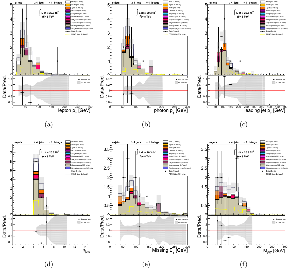
FIGURE 50. Lepton p_T (a), photon p_T (b), leading jet p_T (c), N_{jets} (d), E_T^{miss} (e), and m_T^W (f) distributions in the t\bar{t} + \gamma validation region (electron channel). FCNC signal BR( t \rightarrow q\gamma ) is scaled to 0.1%.
