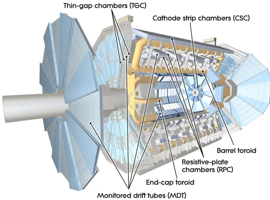
FIGURE 28. The ATLAS muon system [41]
