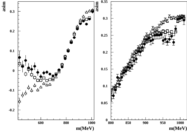
Fig. 5. Charge asymmetry data (full circles) compared to a simulation based on the non scalar part of the spectrum only (open triangles) and on the non-scalar part plus the f_0 part obtained from the kaon-loop amplitude (open squares). The plot on the right shows the detail of the comparison in the f_0 region.
