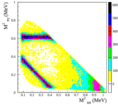
Fig. 6. Dalitz plot distribution ( m_{\pi^0\gamma}^2 versus m_{\pi^0\pi^0}^2 ) of the \pi^0\pi^0\gamma events.
