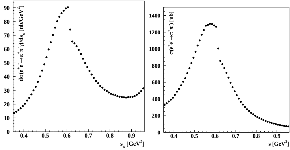
Fig. 3. Left: KLOE measurement for d\sigma(e^+e^- \rightarrow \pi^+\pi^-\gamma)/ds_\pi , inclusive in \theta_\pi and with \sin\theta_\gamma < \sin 15^\circ . Right: bare cross section for e^+e^- \rightarrow \pi^+\pi^- .
