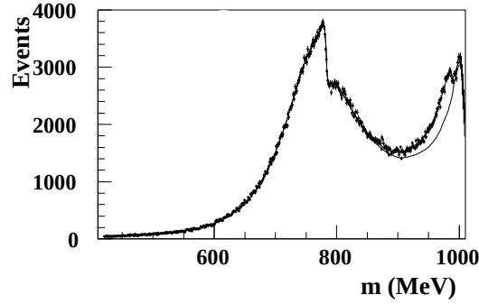
Fig. 4. M_{\pi\pi} spectrum for e^+e^- \rightarrow \pi^+\pi^-\gamma . Data are compared with the fitting function (upper curve following the data points) and with the estimated non-scalar part of the function (lower curve). The fit uses the kaon-loop model for the f_0 .
