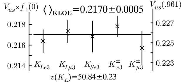
Fig. 2. |V_{us}f_+(0)| measurements. For K_L BR the KLOE \tau_L has been used.
