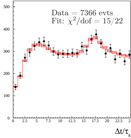
Fig. 1. Fit of the difference \Delta t of the decay times of K_S \rightarrow \pi^+ \pi^- and K_L \rightarrow \pi^+ \pi^- . The full circles are data and the histogram is the result of the fit. The peak at \Delta t \sim 17\tau_S is due to the regeneration on the beam pipe.
