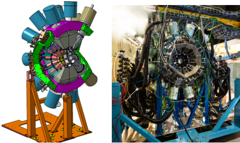
Fig. 1. (Colour on-line) Left — CAD drawing of half of the \nu -ball array. \text{LaBr}_3 detectors are black/pink. On their right, the BGO shields of the clover detectors are drawn. Phase I HPGe detectors are symmetric to \text{LaBr}_3 , with respect to clovers. Right — a photo of the \nu -ball array before the commissioning experiment is presented.
