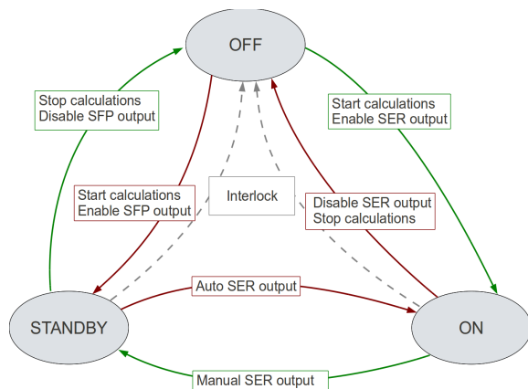
Figure 5: Simplified FOFB state diagram.
