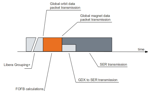
Figure 7: Time portions in the FOFB cycle.
