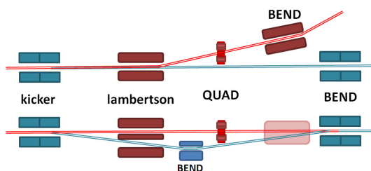
Figure 7: The layout of the beam distribution system.
