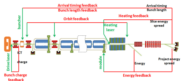
Figure 8: The layout of the injector feedback system.
