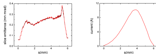
Figure 5: Slice parameters of the electron beam at injector exit.
