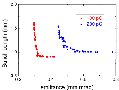
Figure 2: Multi-objective optimization results of the injector.
