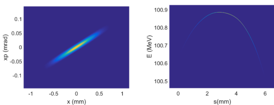
Figure 4: The longitudinal phase distribution of the electron beam at the injector exit.
