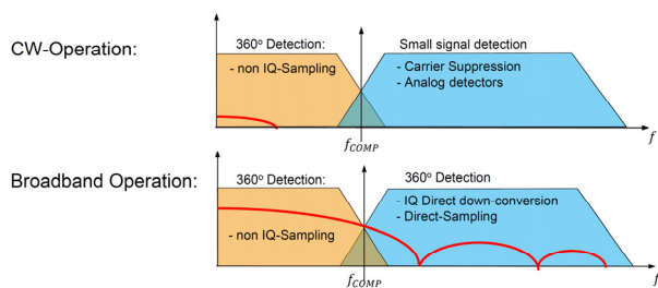
Figure 8: Down conversion hybrid options.
