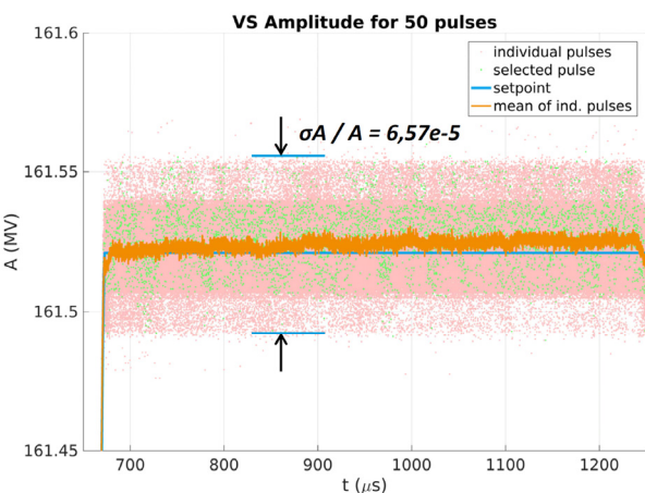
Figure 4: Amplitude in-loop performance at FLASH.
