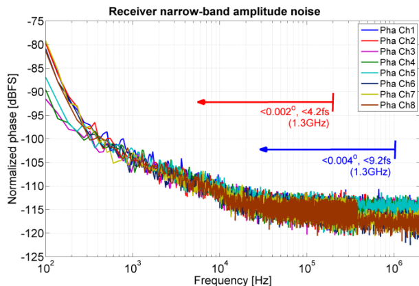
Figure 1: Field detector narrow-band phase noise with 0.002 deg, 4.2 fs (100 Hz - 200 kHz), respectively 0.004 deg, 9.2 fs(100Hz - 1 MHz) @ 1.3 GHz.
