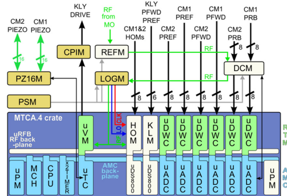
Figure 2: Schematic of a LLRF system of the Eu-XFEL.
