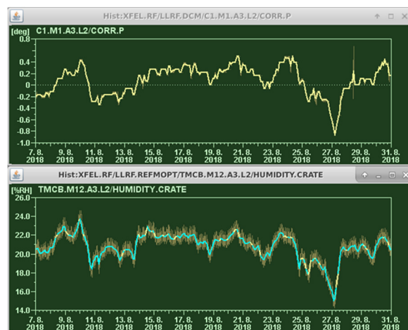
Figure 5: EuXFEL phase corrections of a LLRF station (top) and humidity changes (bottom) over a period of 3 weeks.
