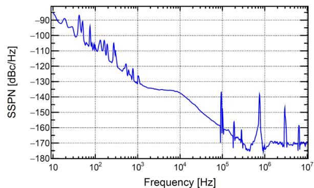
Figure 3: Cavity phase noise spectrum at ELBE.
