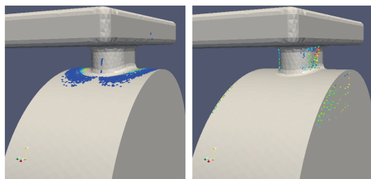
Figure 5: Resonant electron trajectories for B = 0 (left) and B = 3 Tesla (right) near the coupler of the modular cavity.
