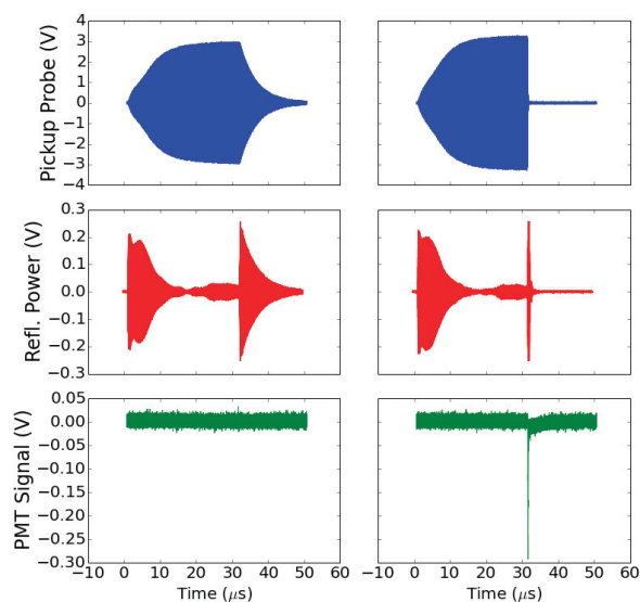
Figure 6: Waveforms recorded for the modular cavity: pickup probe voltage (blue), reflected power from directional coupler (red), and visible light via optical fiber and PMT (green). The left column shows a normal pulse, while the right column shows a pulse during RF breakdown, captured by the DAQ.
