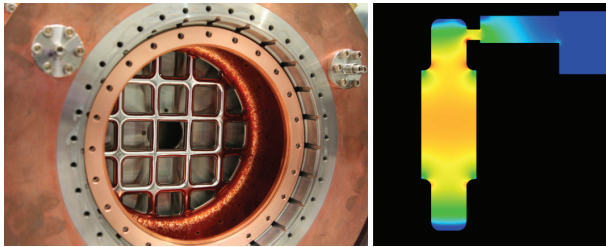
Figure 2: An 805 Mhz pillbox cavity with windows composed of a grid of tubes (left) and electric field of the TM_{010} mode (right), simulated using SLAC's ACE3P RF code suite.
