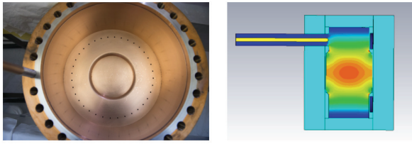
Figure 1: All-Seasons cavity interior (left) and electric field of the TM_{010} mode (right), simulated using CST Microwave Studio. Note the bolts and RF seal region in the left-hand photo.
