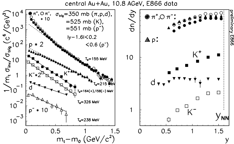
Fig.1. Data from E866. Left: Boltzmann representation of spectra measured around midrapidity in central Au+Au collisions. T_B denotes the inverse slope parameter. Right: rapidity distributions, shown in one hemisphere. Besides pion and proton distributions data is preliminary. Statistical errors only, systematic errors estimated to be \pm(10 - 15)\% .
