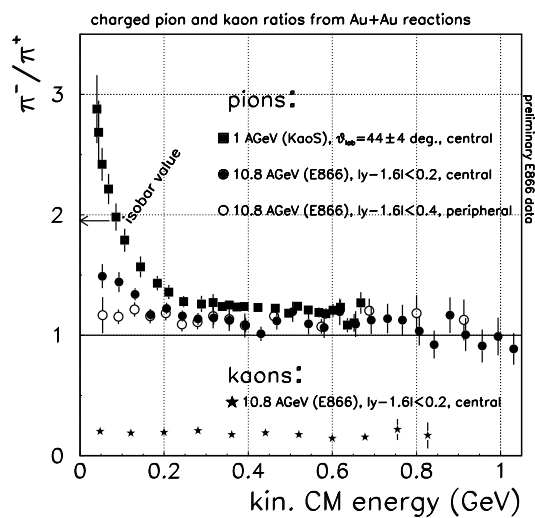
Fig. 2. Energy differential ratios of spectral distribution of positively and negatively charged pions and kaons at 1 and 10.8 AGeV incident energy [6, 2]. Preliminary data, besides the pion data at central reactions. Statistical errors only.
